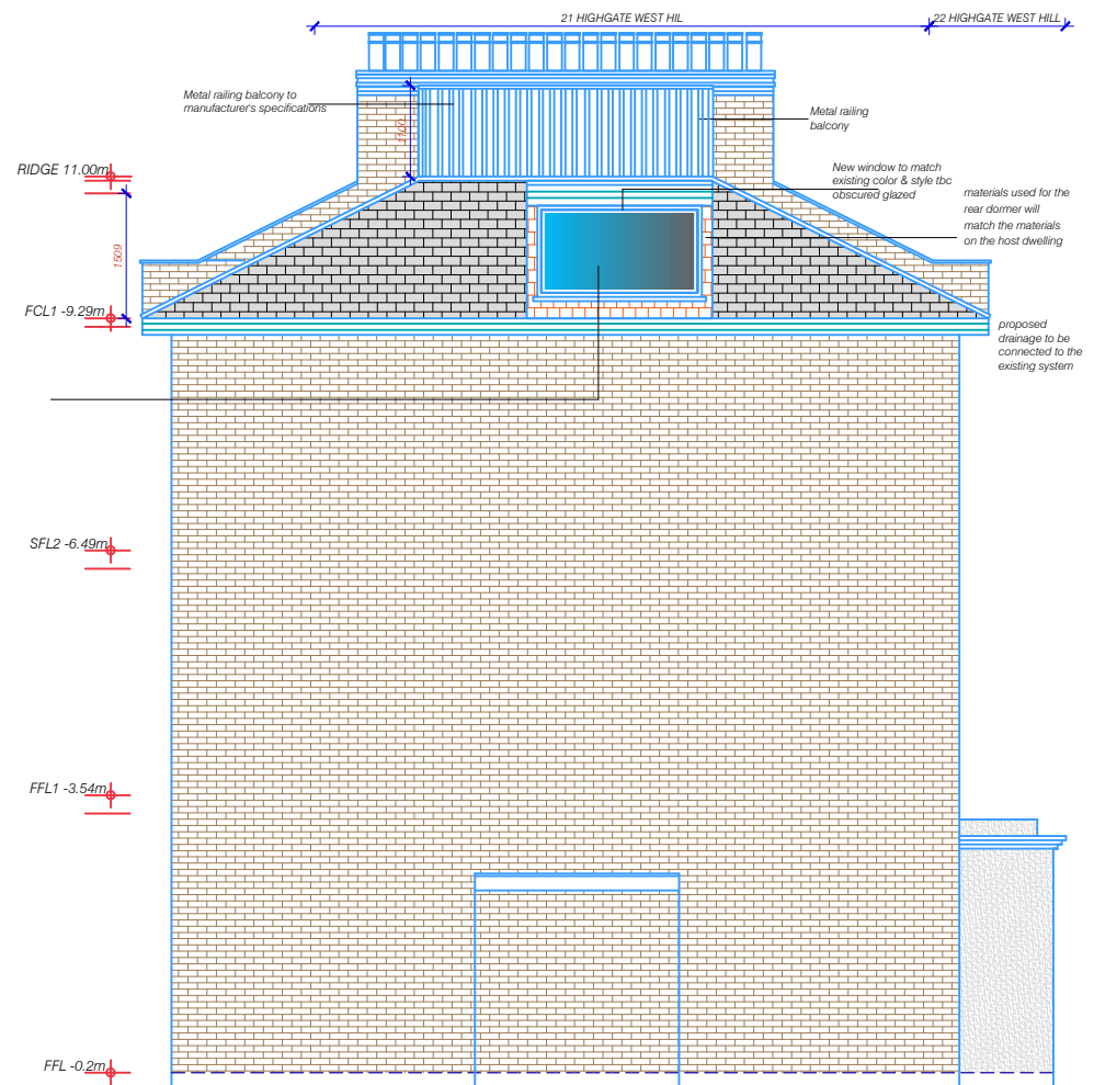
PROPOSED SIDE ELEVATION A
