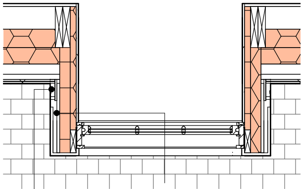
Provide continuous air paths for dormer ventilation.
