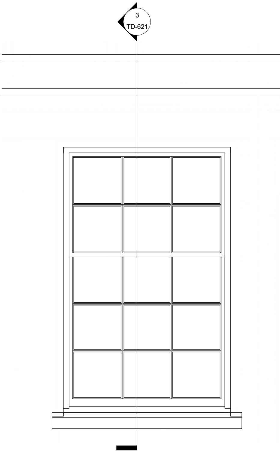
Typical Window Elevation - Type A
