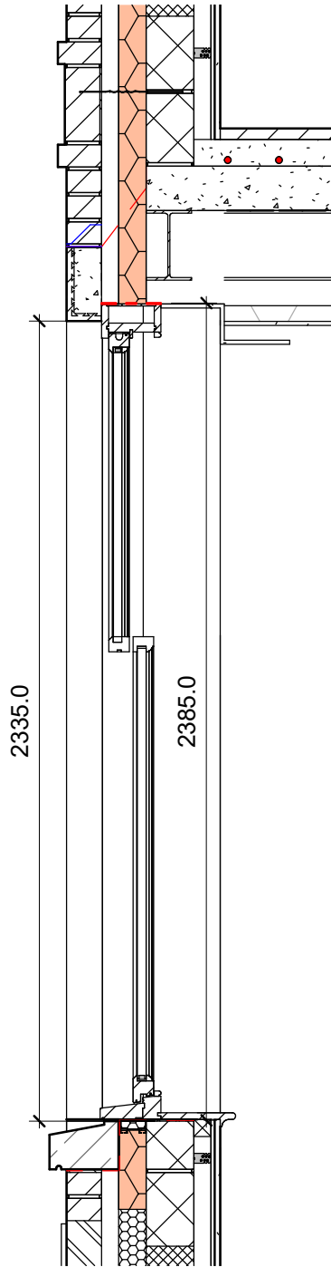
Typical Window Section - Type A
