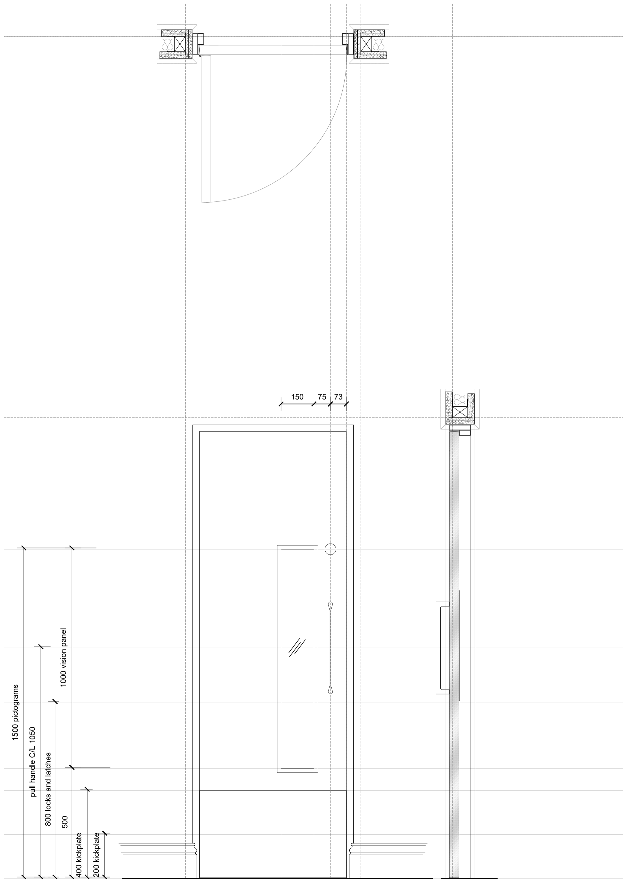
13 DOOR TYPE 13 HYGIENIC SINGLE DOOR 1:10 GRP DOOR WITH VISION PANEL TYPE S JAMB
