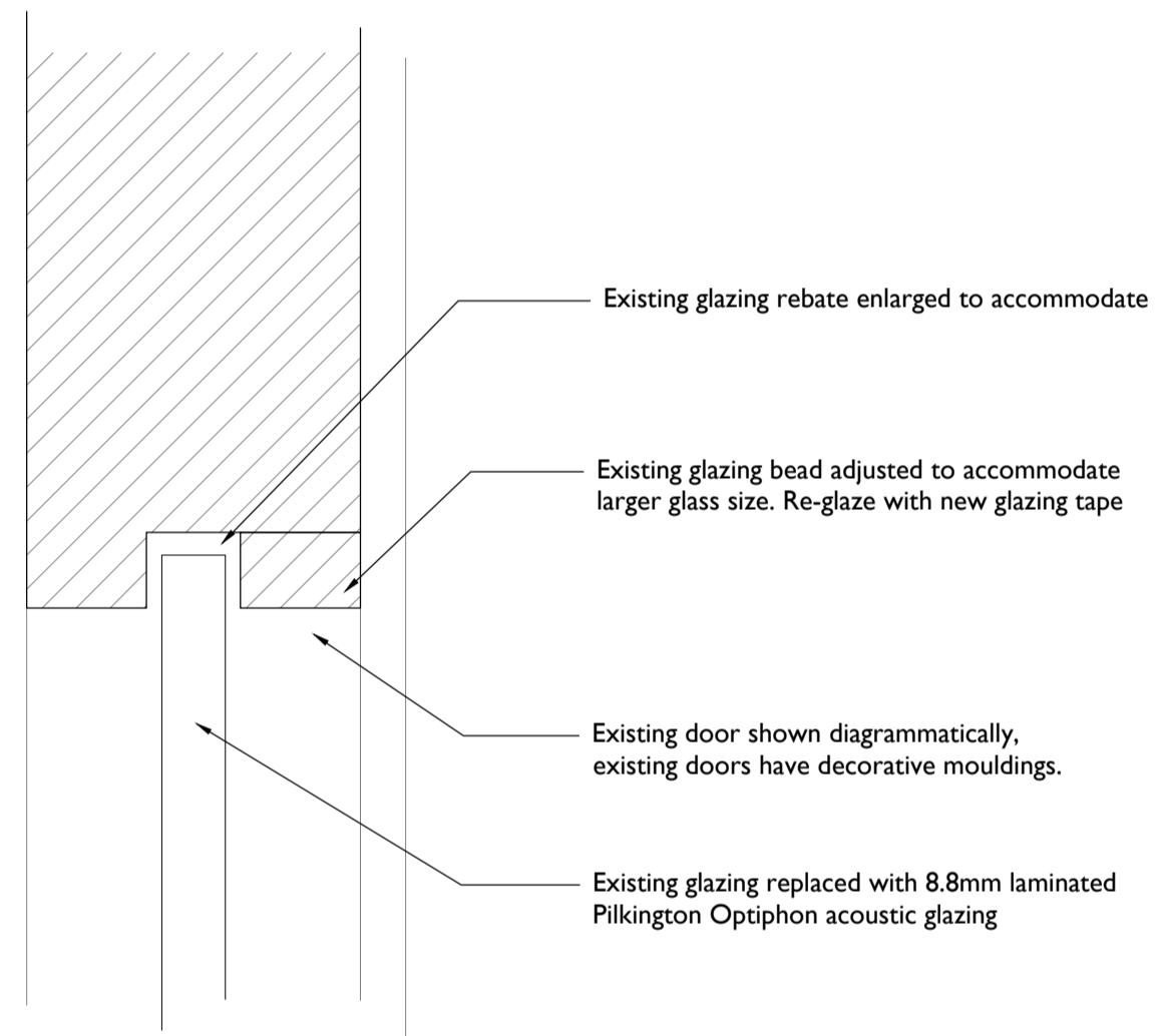
3 DOOR GLAZING DETAIL 1:1
