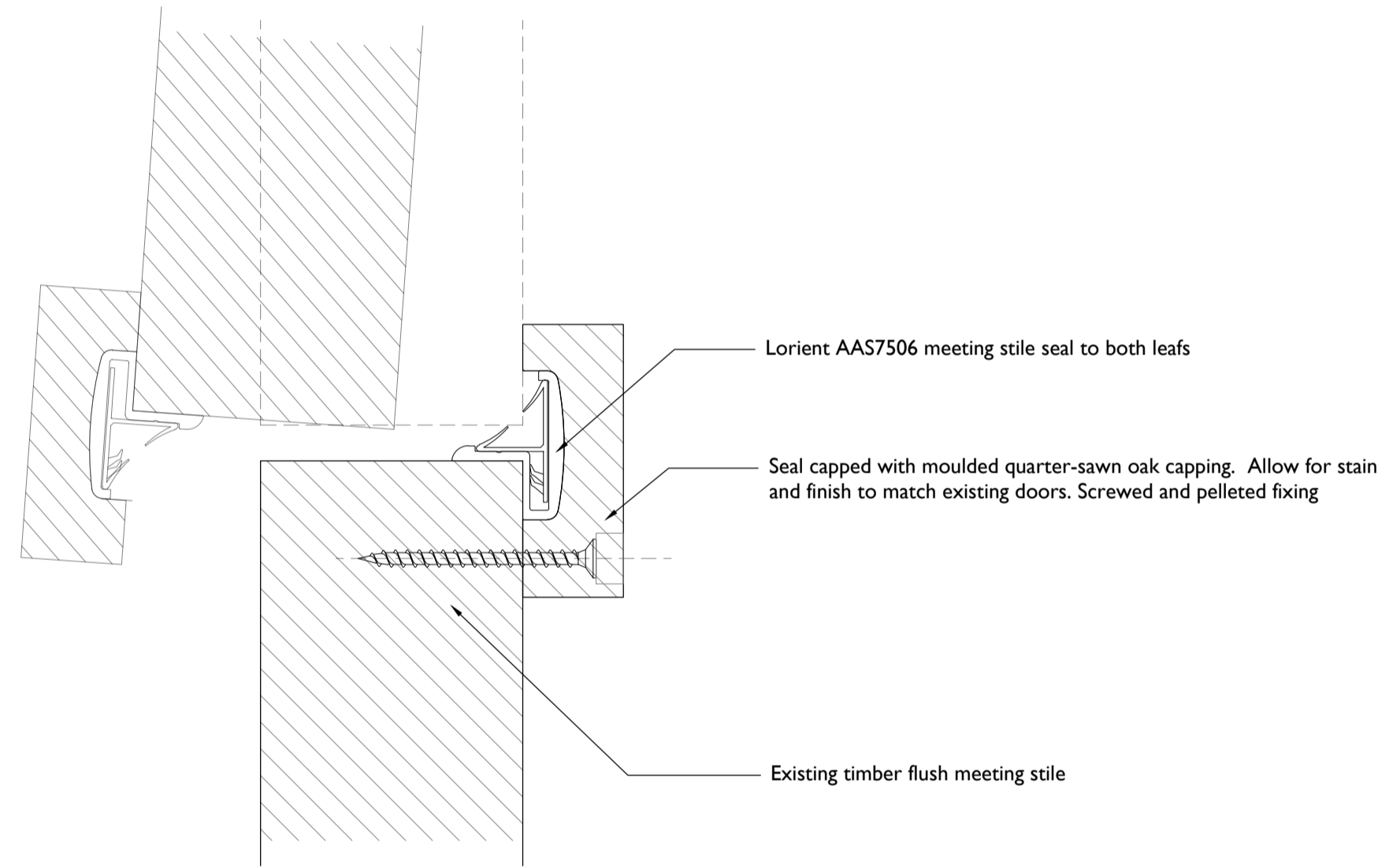
4 MEETING STILE DETAIL 1:1
