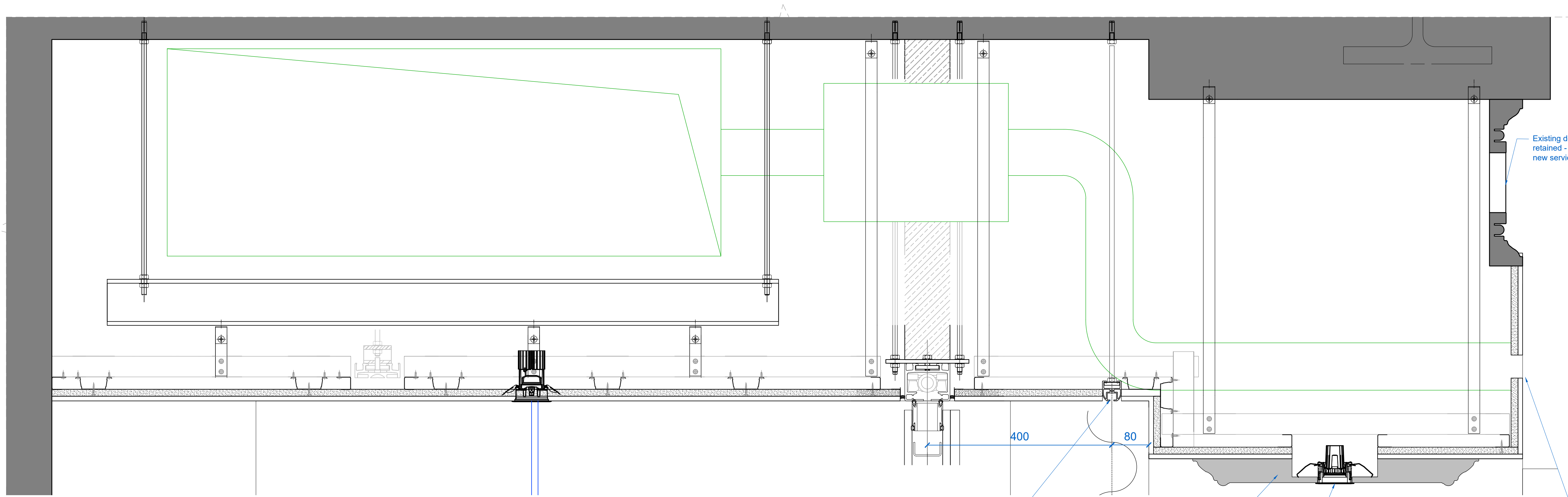
1 EVENT SPACE FOLDING PARTITION HEAD DETAIL 6006 1:5
