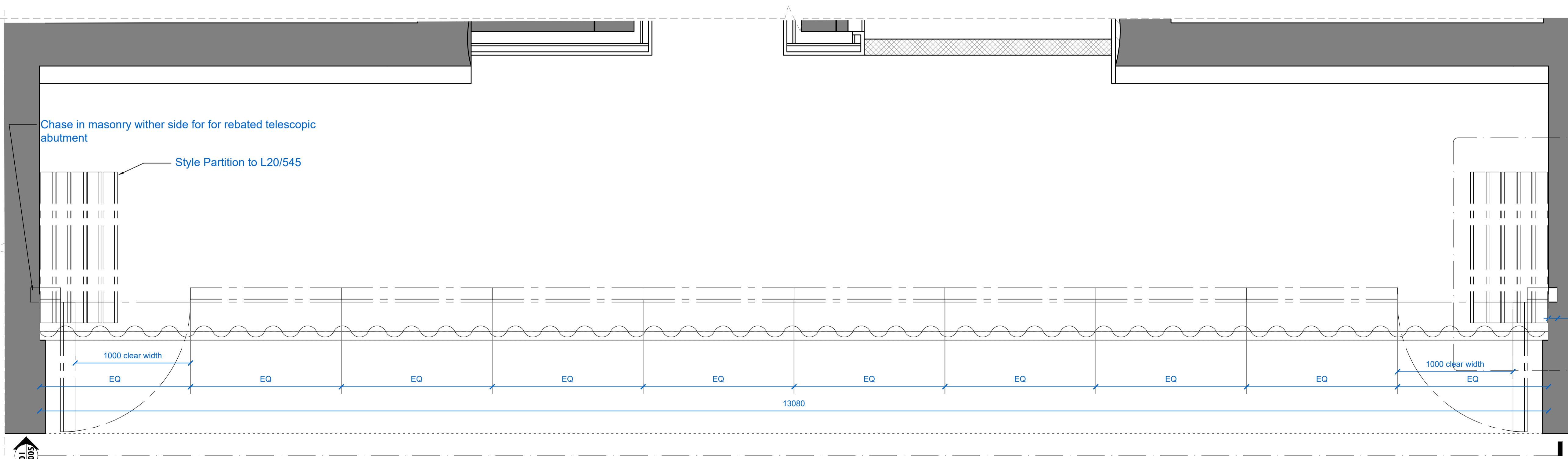
2 EVENT SPACE FOLDING PARTITION PLAN 6005 1:20
