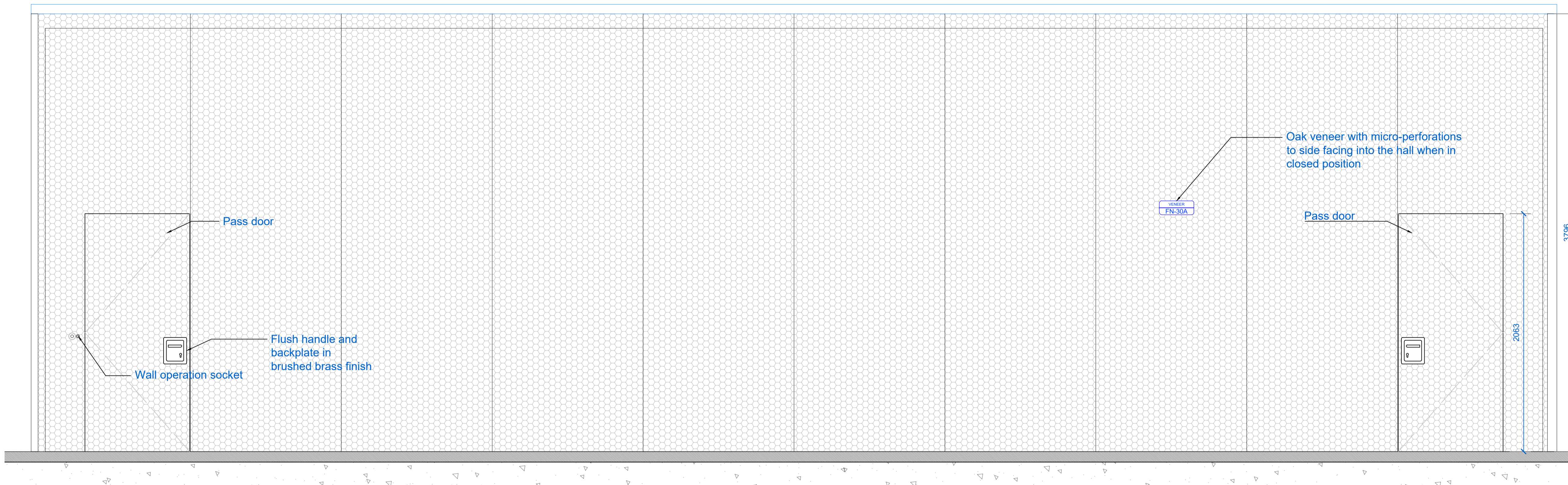
1 EVENT SPACE FOLDING PARTITION ELEVATION 6005 1:20
