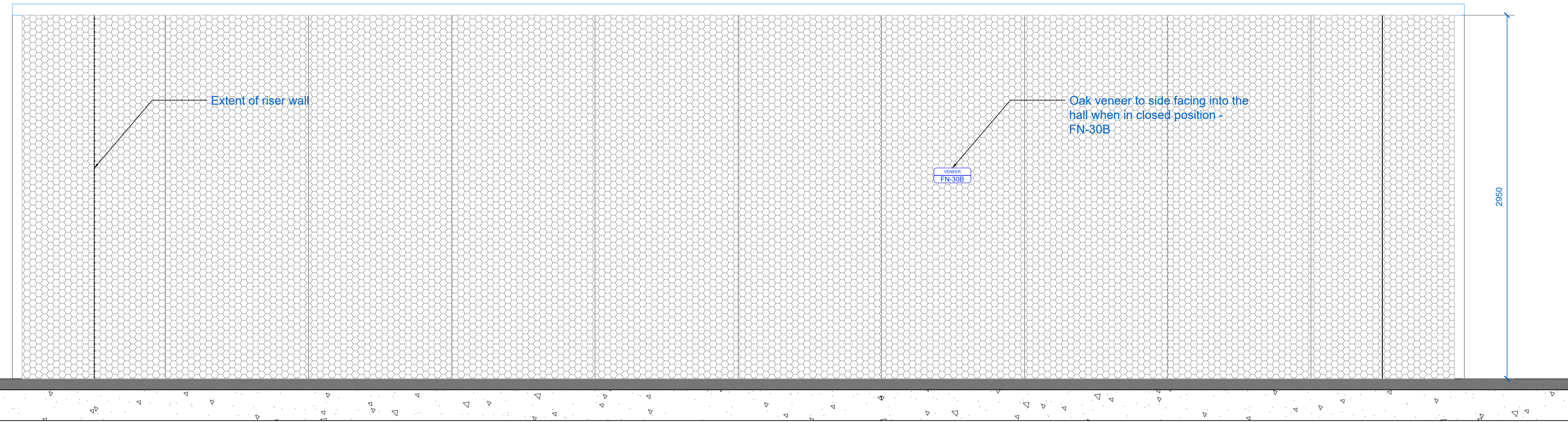
1 L01 GALLERY PARTITION ELEVATION 6004 1:20
