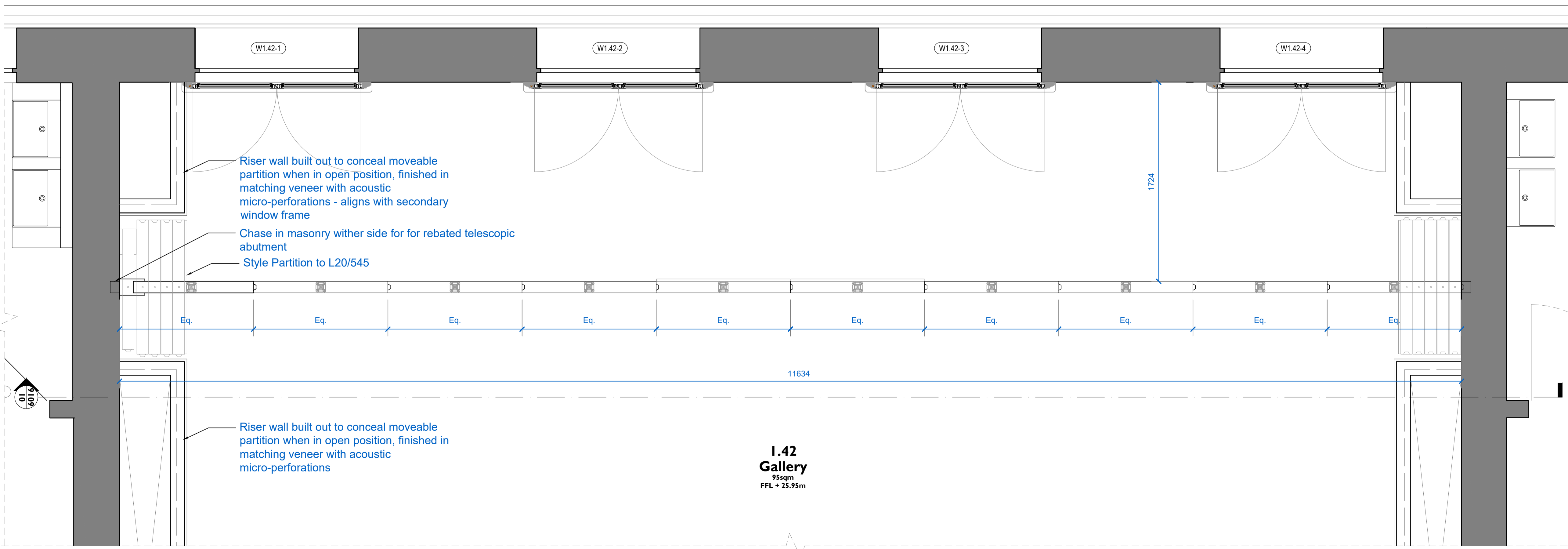
2 L01 GALLERY FOLDING PARTITION PLAN 6004 1:20
