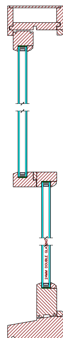
PROPOSED SECTION A-A SCALE 1:2
