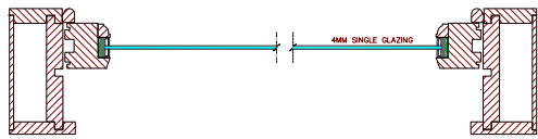
EXISTING SECTION B-B SCALE 1:2
