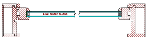
PROPOSED SECTION B-B SCALE 1:2
