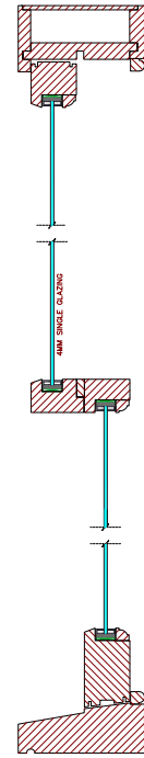
EXISTING SECTION A-A SCALE 1:2
