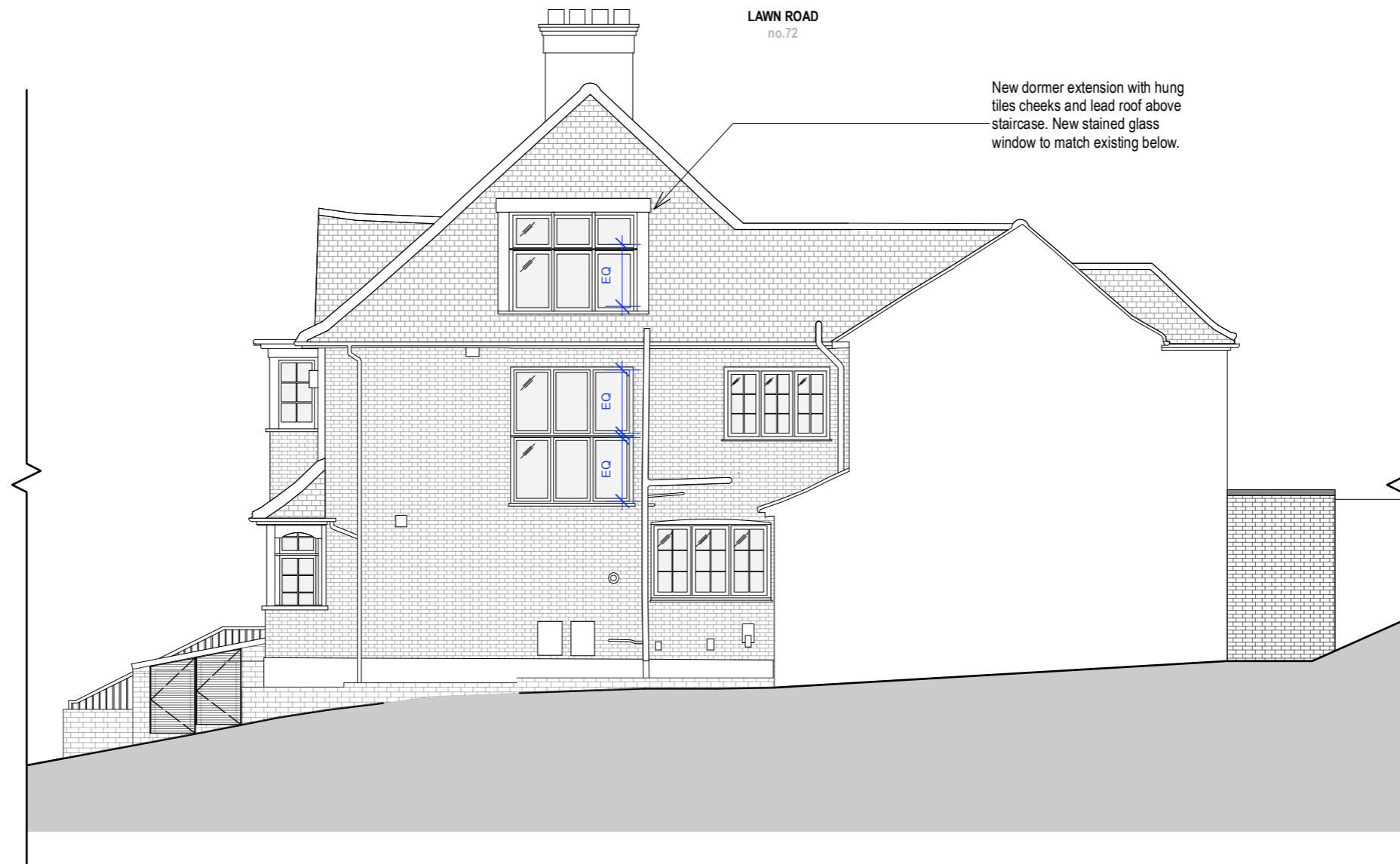
Proposed Elevation - Side (North)
