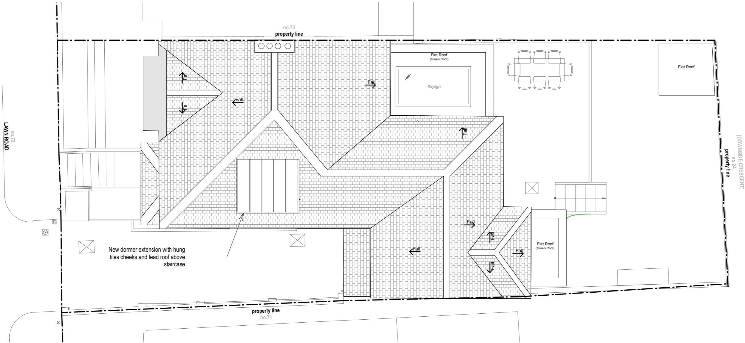
Proposed Plan - Roof 1:100
