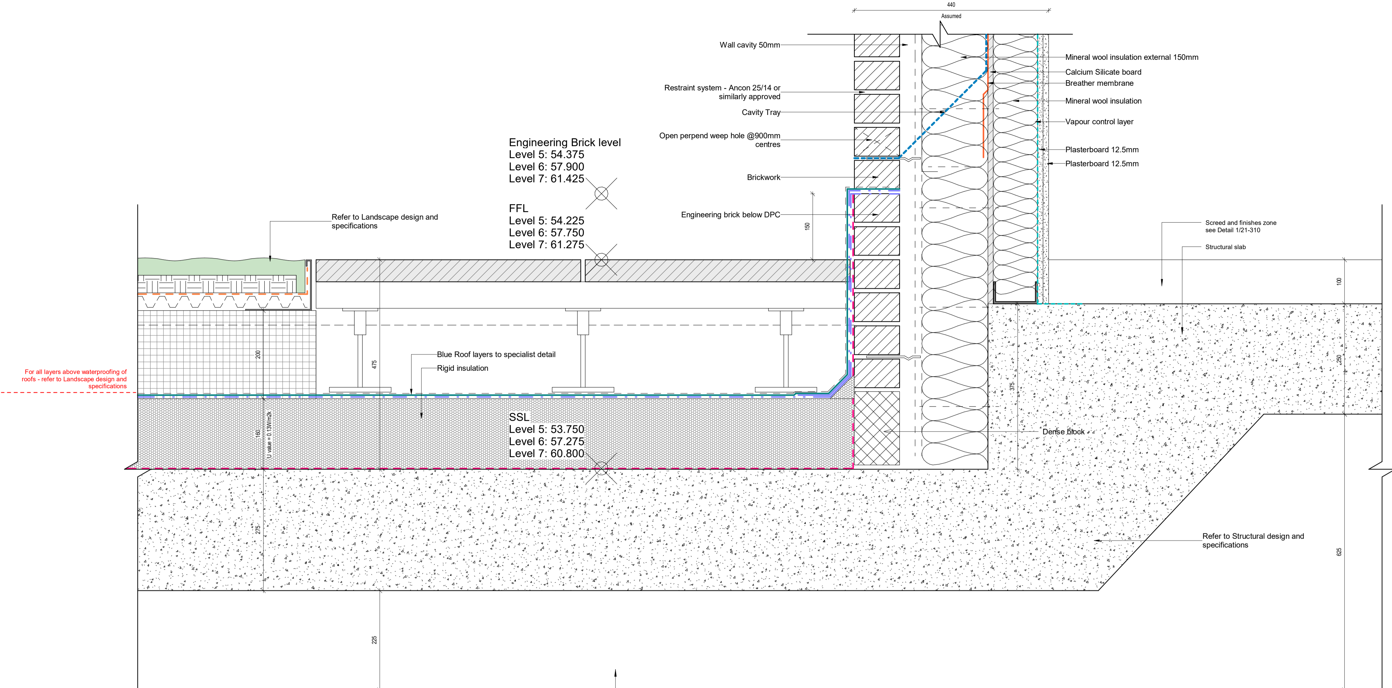
1 Typical Detail Upstand 1 : 5
