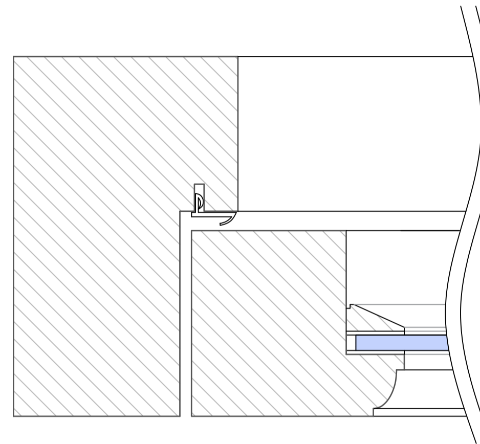
SECTION THROUGH FRAME JAMB SCALE 1:1
