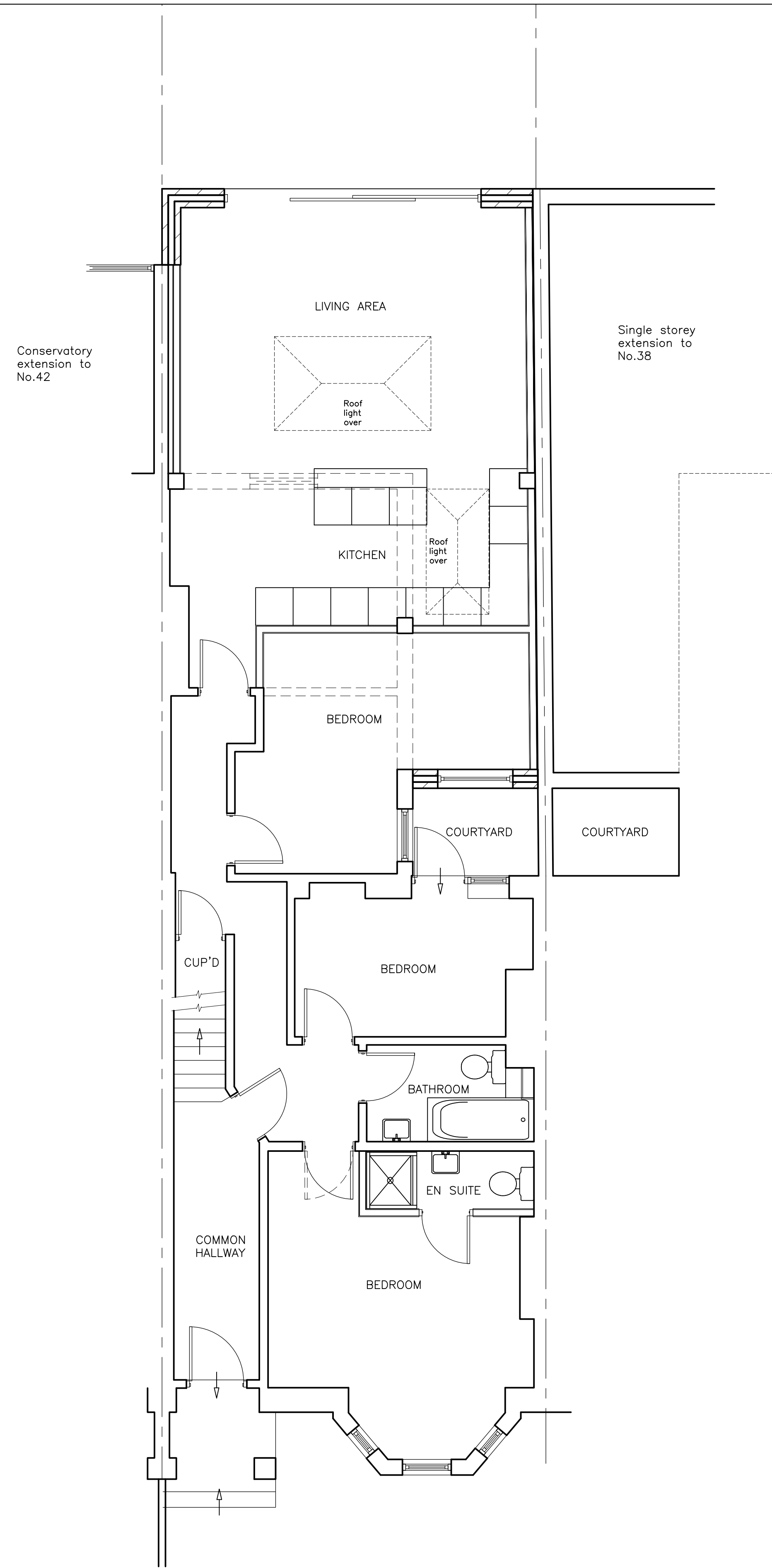
GROUND FLOOR PLAN (1:50)
