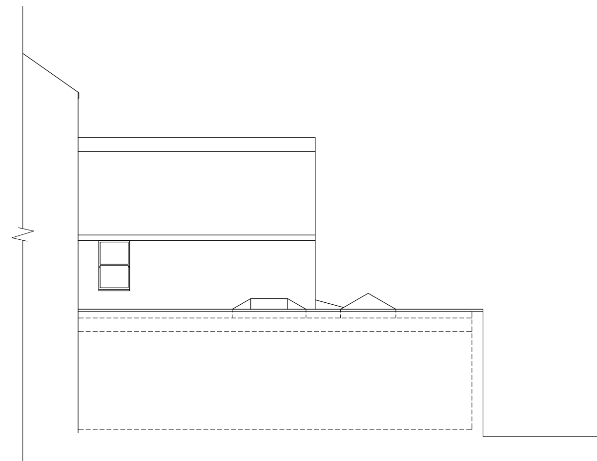
LEFT ELEVATION (1:100)
