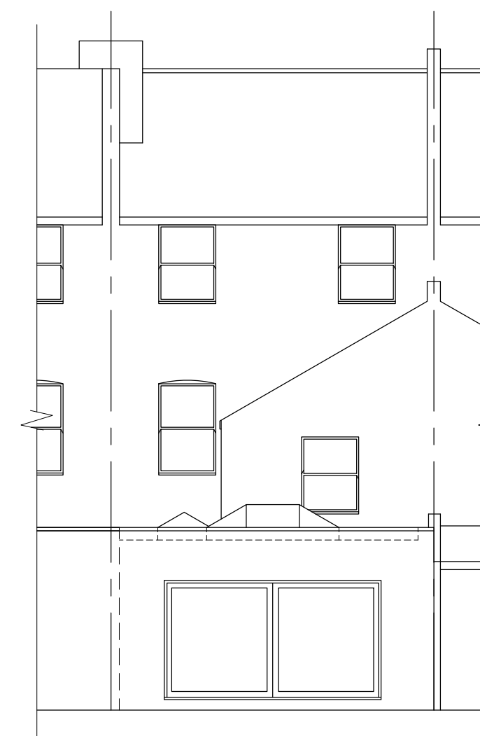
REAR ELEVATION (1:100)
