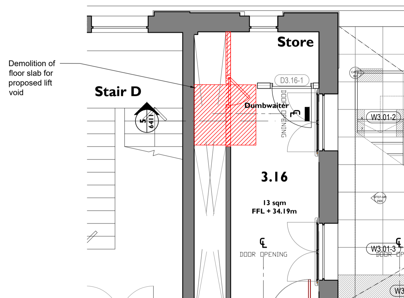
3 3.16 Ice - Demo Plan 6411 1:50 @ A1
