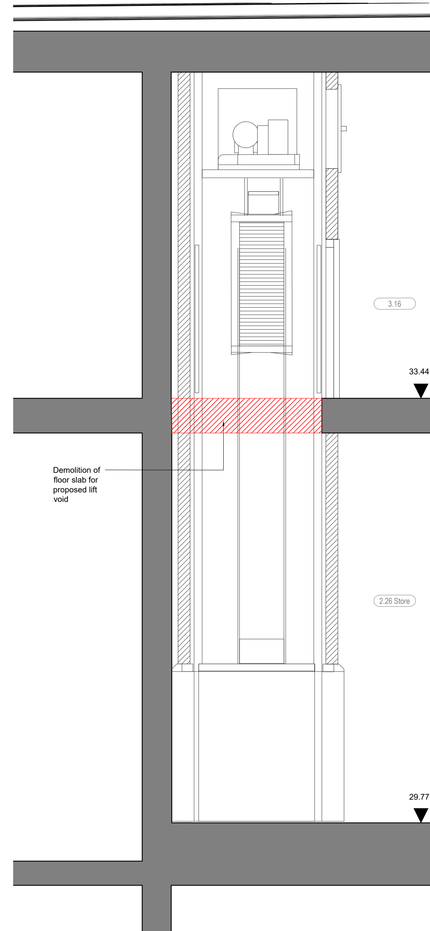
5 Dumbwaiter Section 6411 1:20 @ A1
