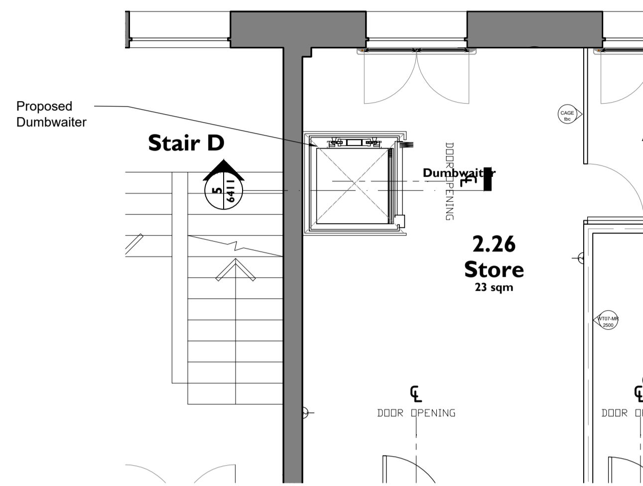
2 2.26 Store - Proposed Plan 6411 1:50 @ A1
