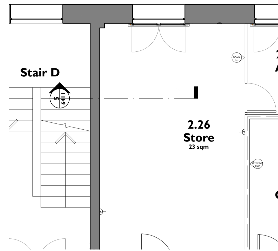
1 2.26 Store - Demo Plan 6411 1:50 @ A1
