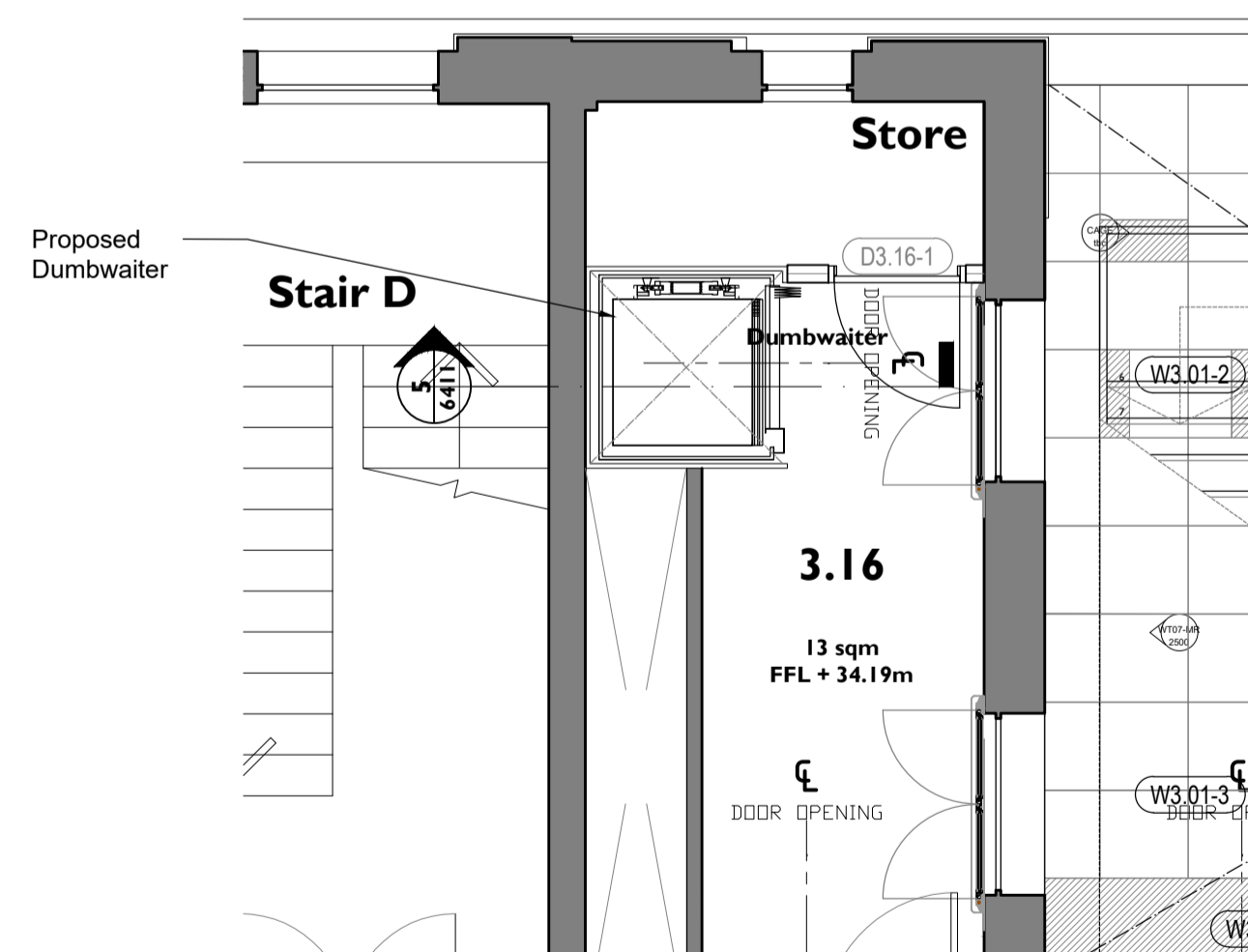
4 3.16 Ice - Proposed Plan 6411 1:50 @ A1
