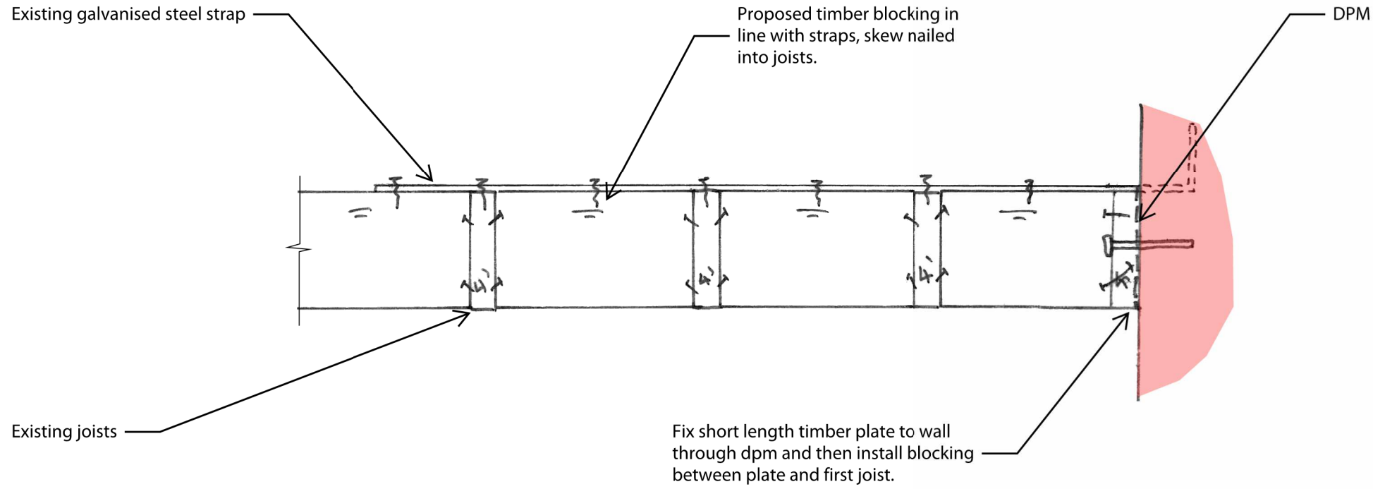
Detail 4-4 - PROPOSED BLOCKING UNDER EXISTING STRAPS
