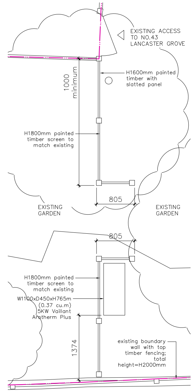
PROPOSED ENLARGED SITE PLAN 2
