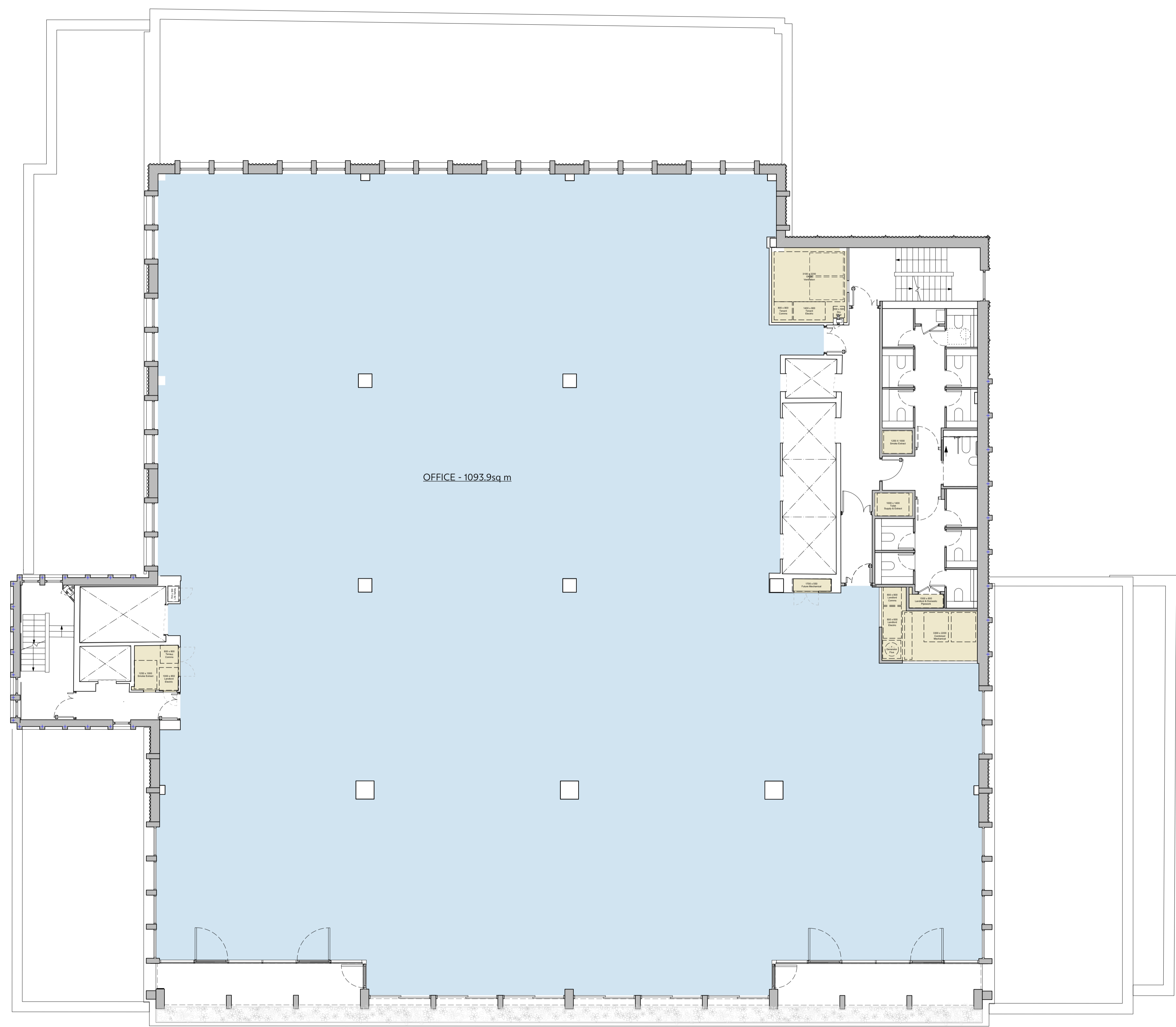
1 Sixth Floor Proposed Plan Scale: 1:100
