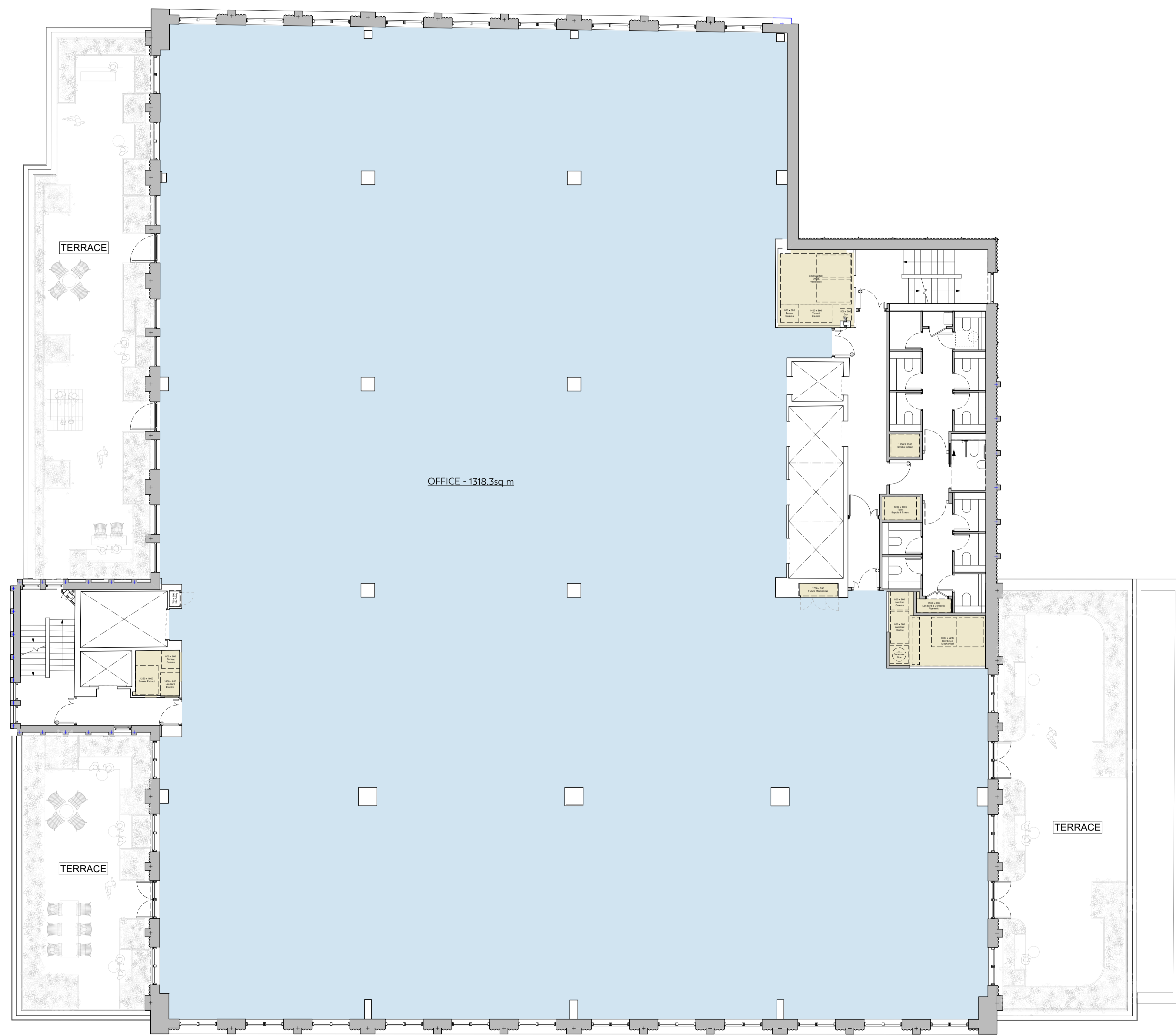
1 Fourth Floor Proposed Plan Scale: 1:100
