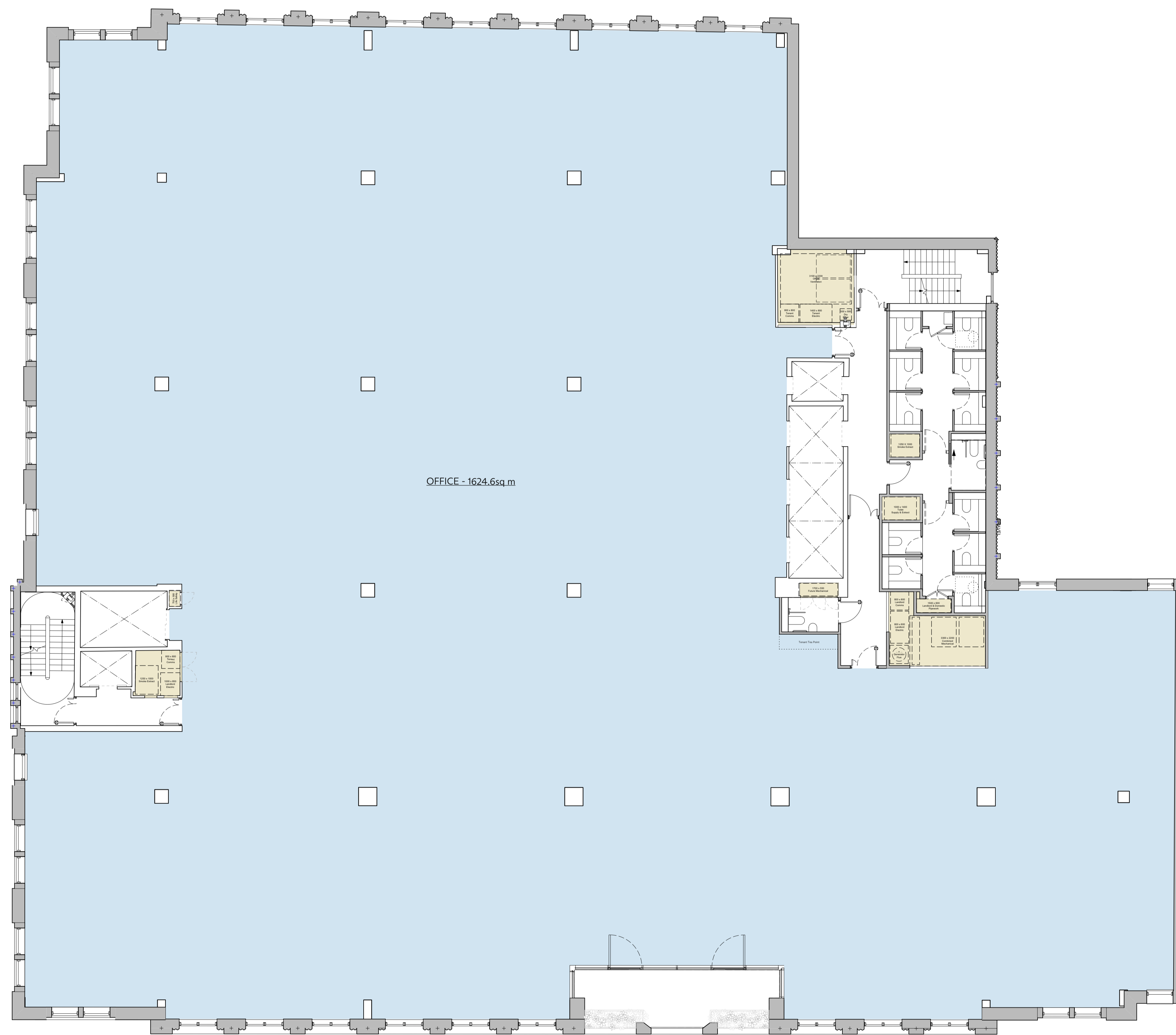
1 Second Floor Proposed Plan Scale: 1:100
