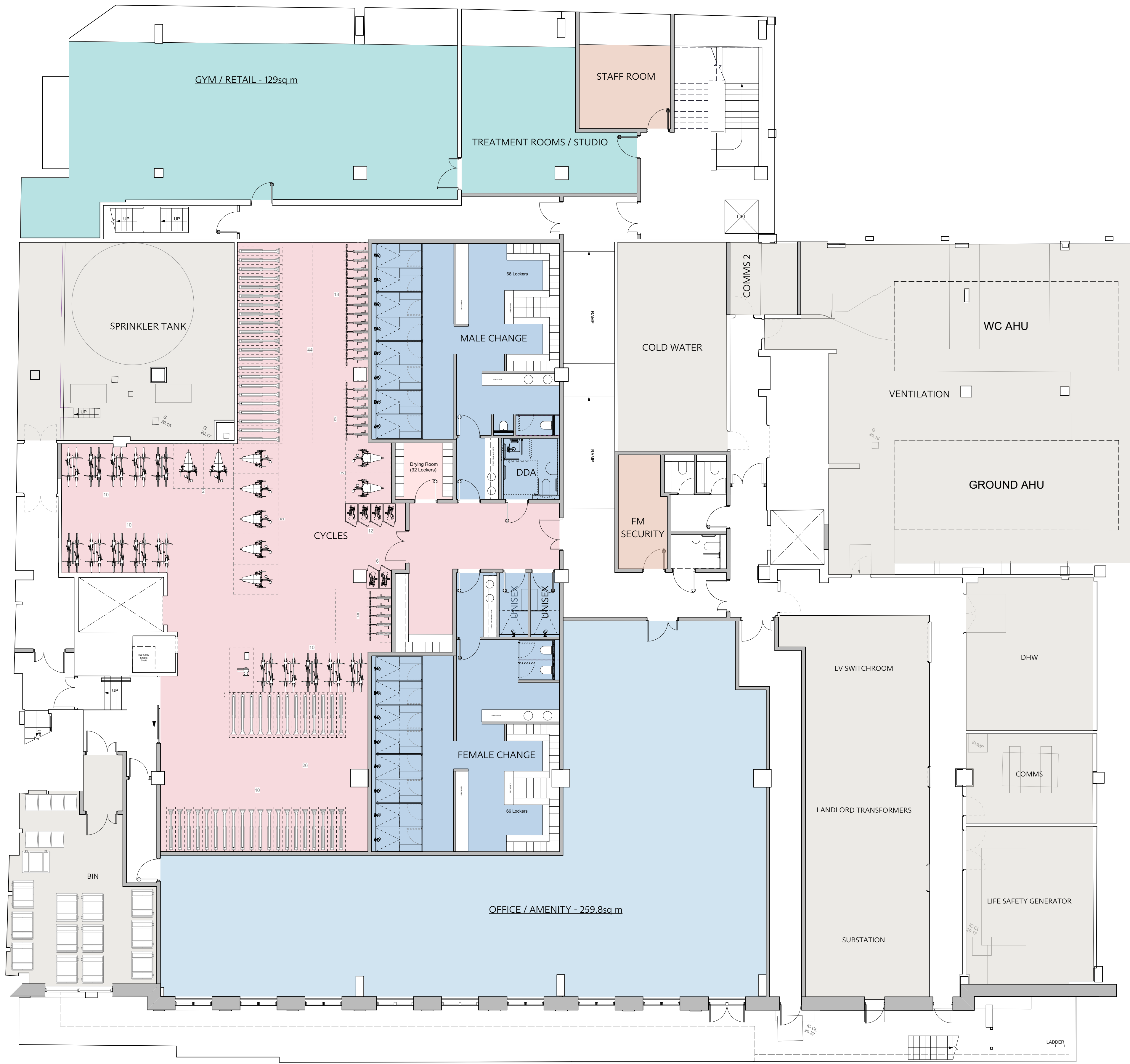
1 Basement Proposed Plan Scale: 1:100
