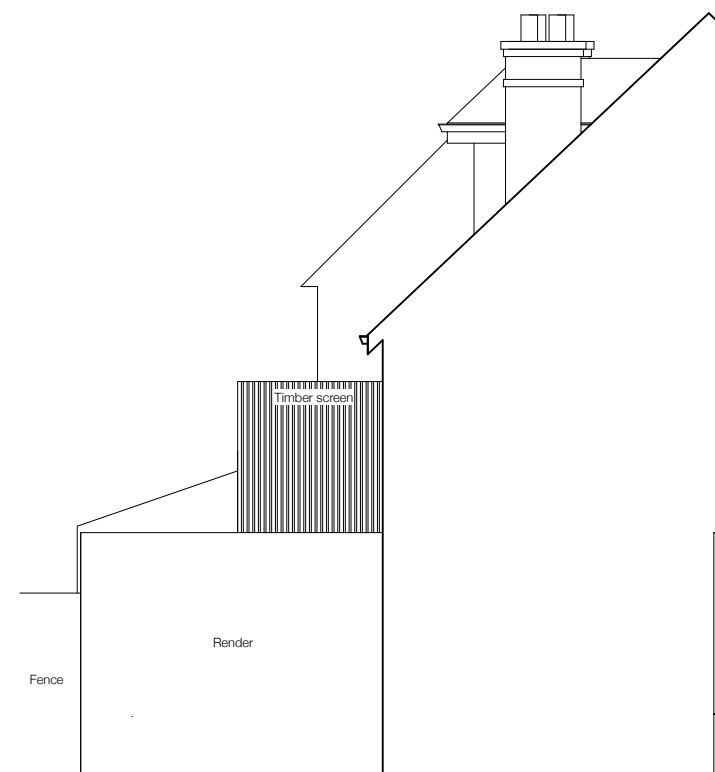
PROPOSED ELEVATION FROM NO. 27
