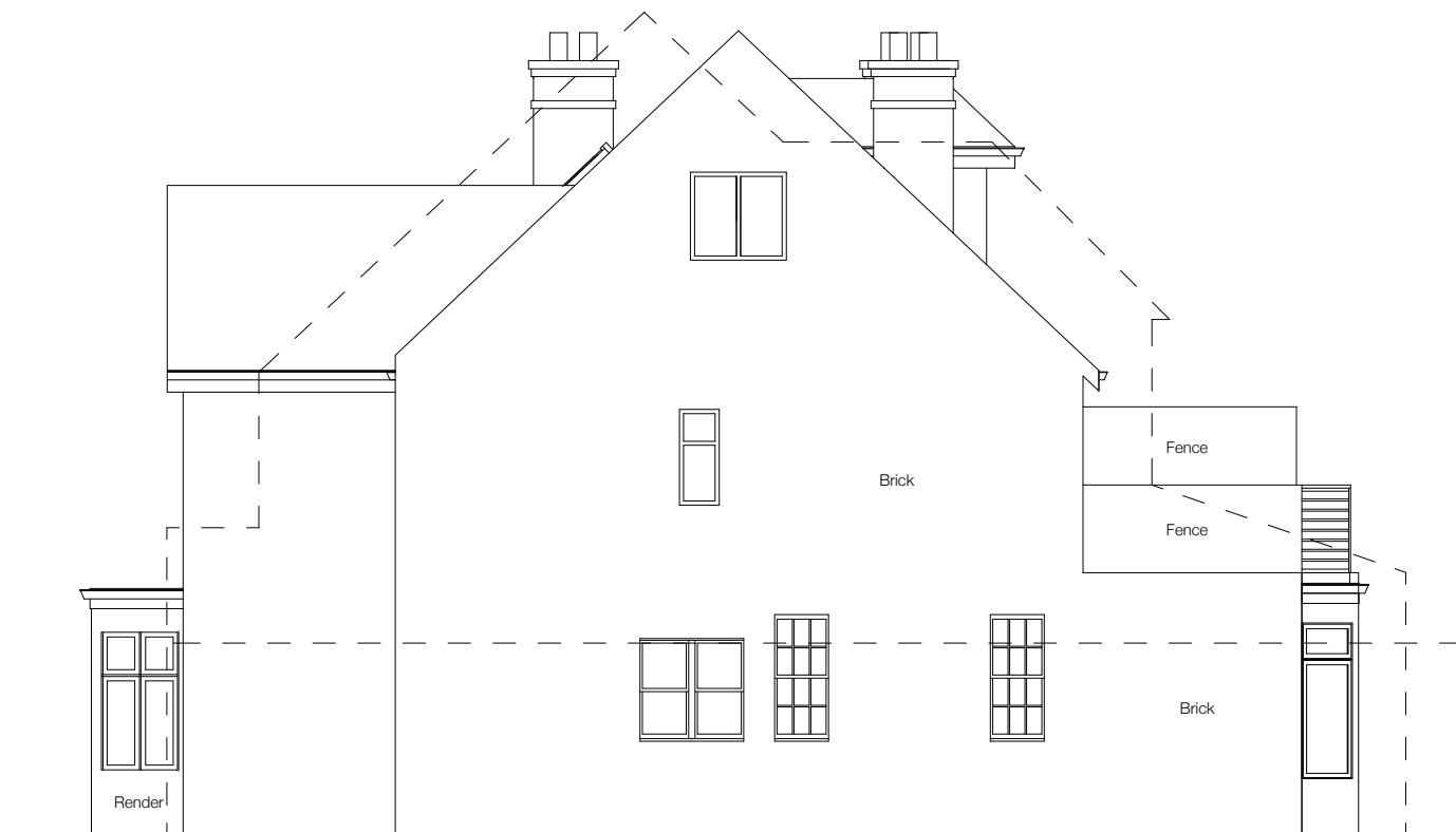
EXISTING ELEVATION FROM SIDE PASSAGE
