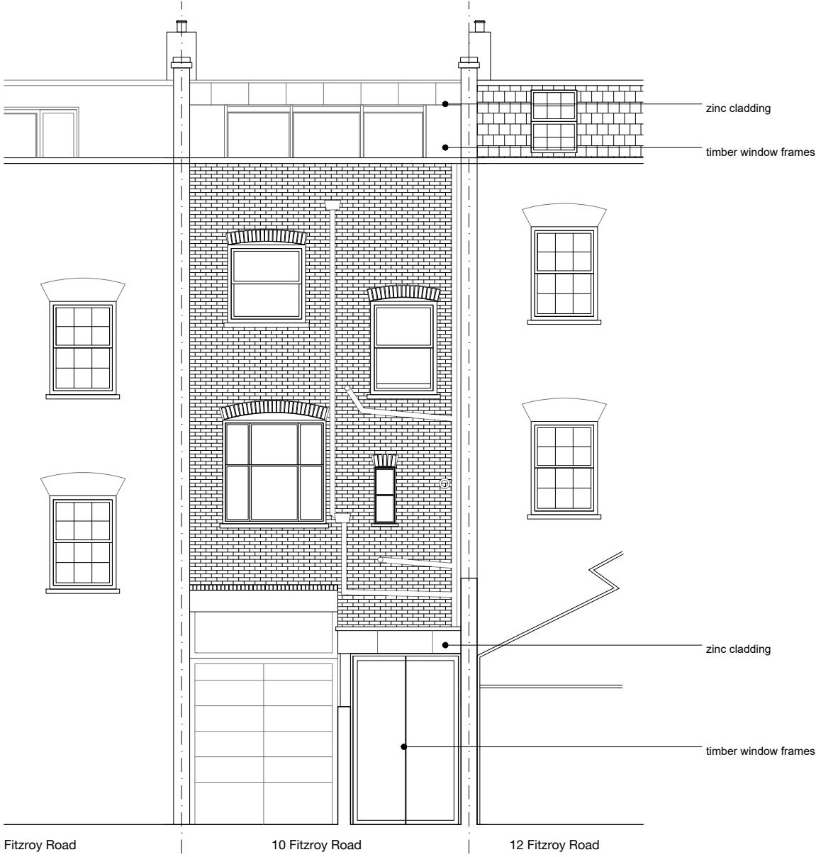
217-(01)250.01 - REAR ELEVATION
