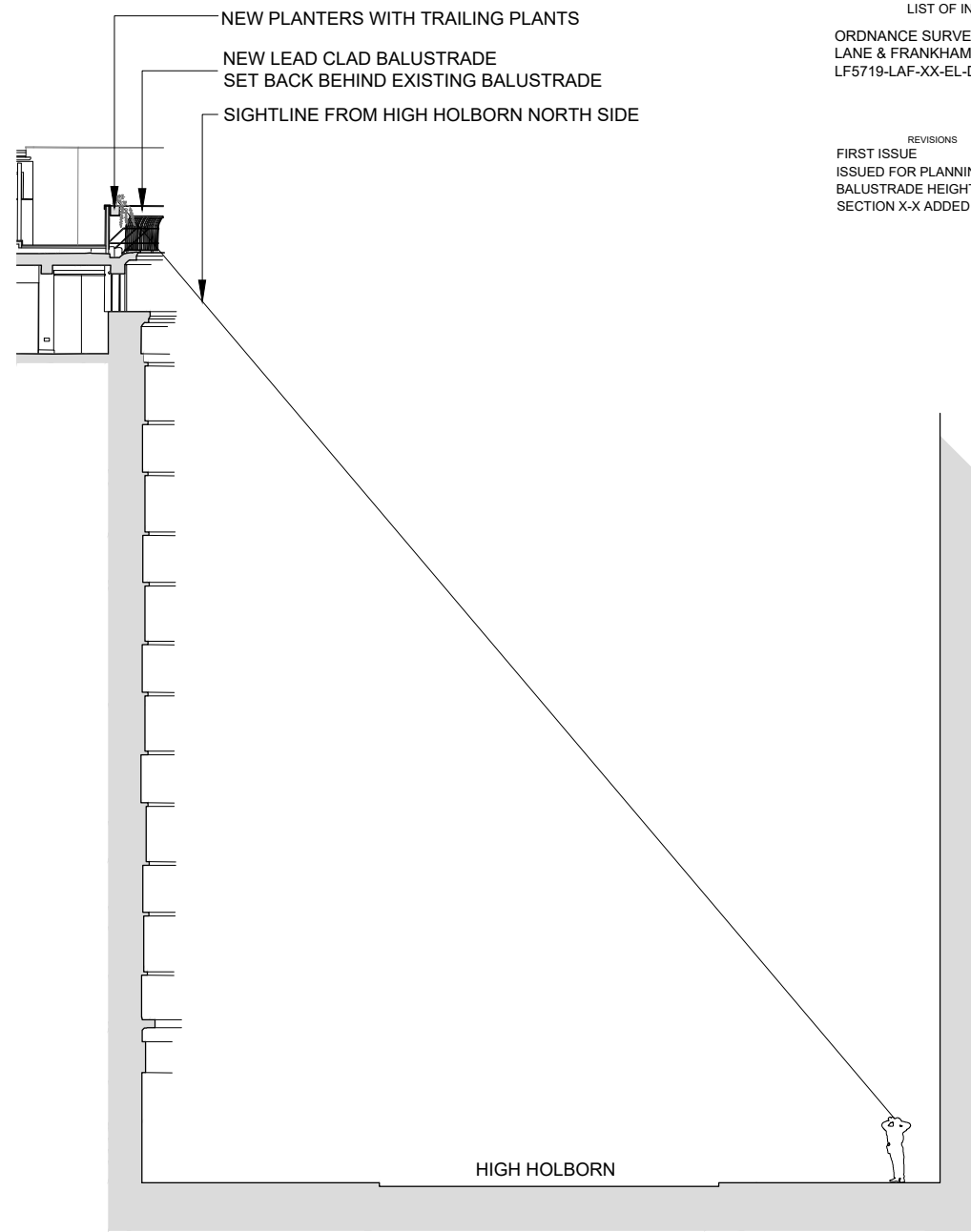
SECTION X-X
