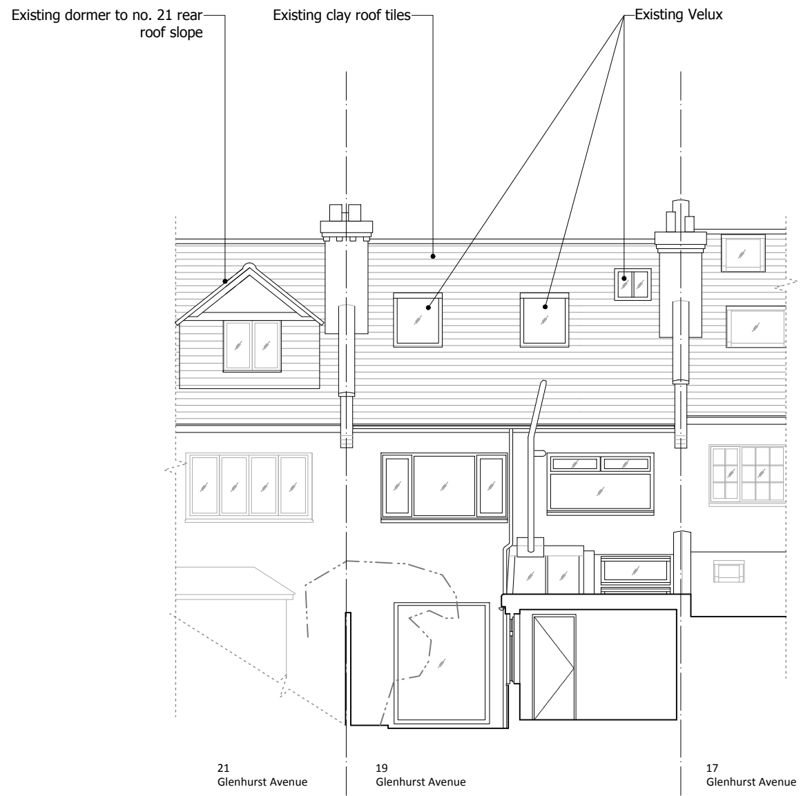
REAR ELEVATION
