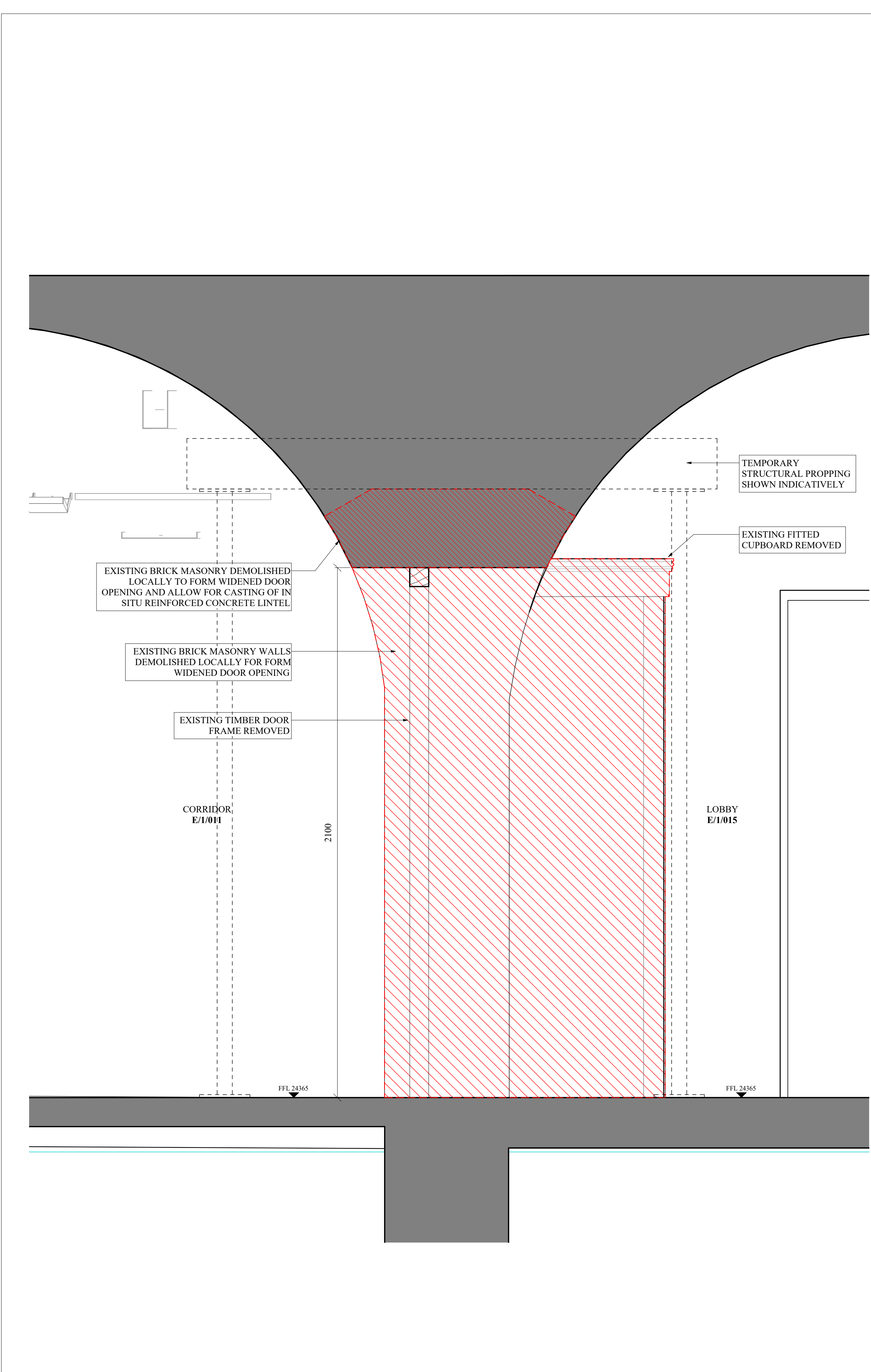
1 Level 1 NE Basement - Door 1 Section - Existing & Demolition
