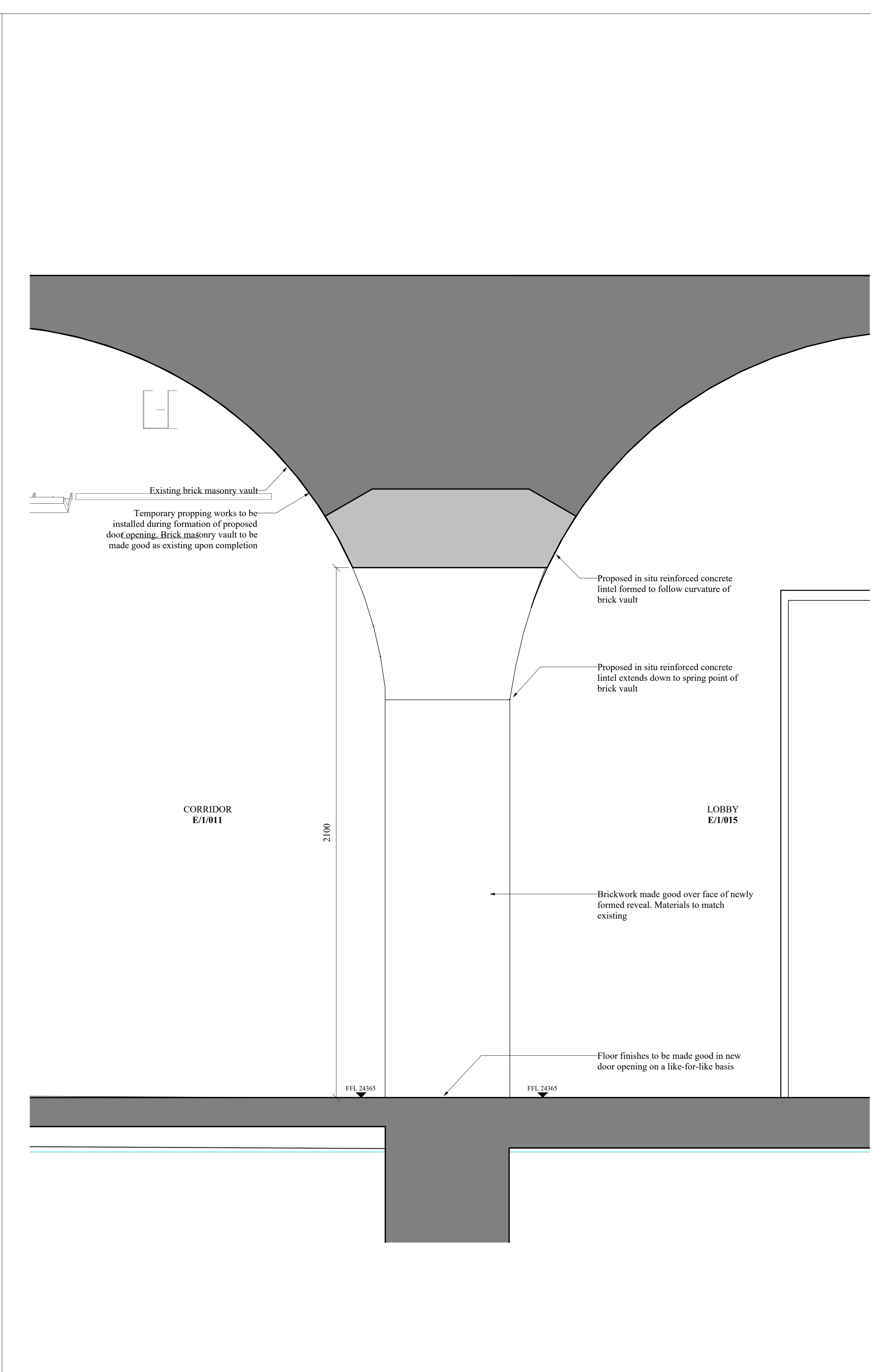
2 Level 1 NE Basement - Door 1 Section - Proposed
