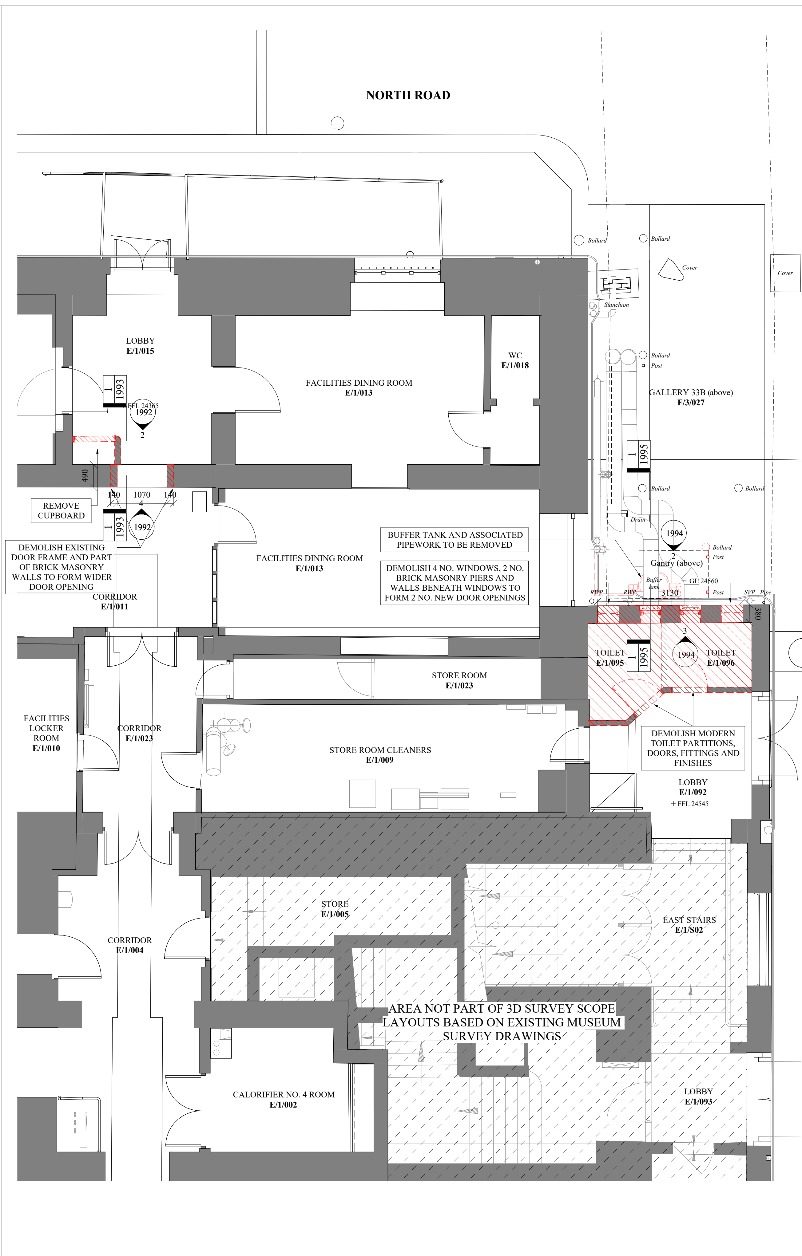
2 Level 1 North-East Plan - Demolition
