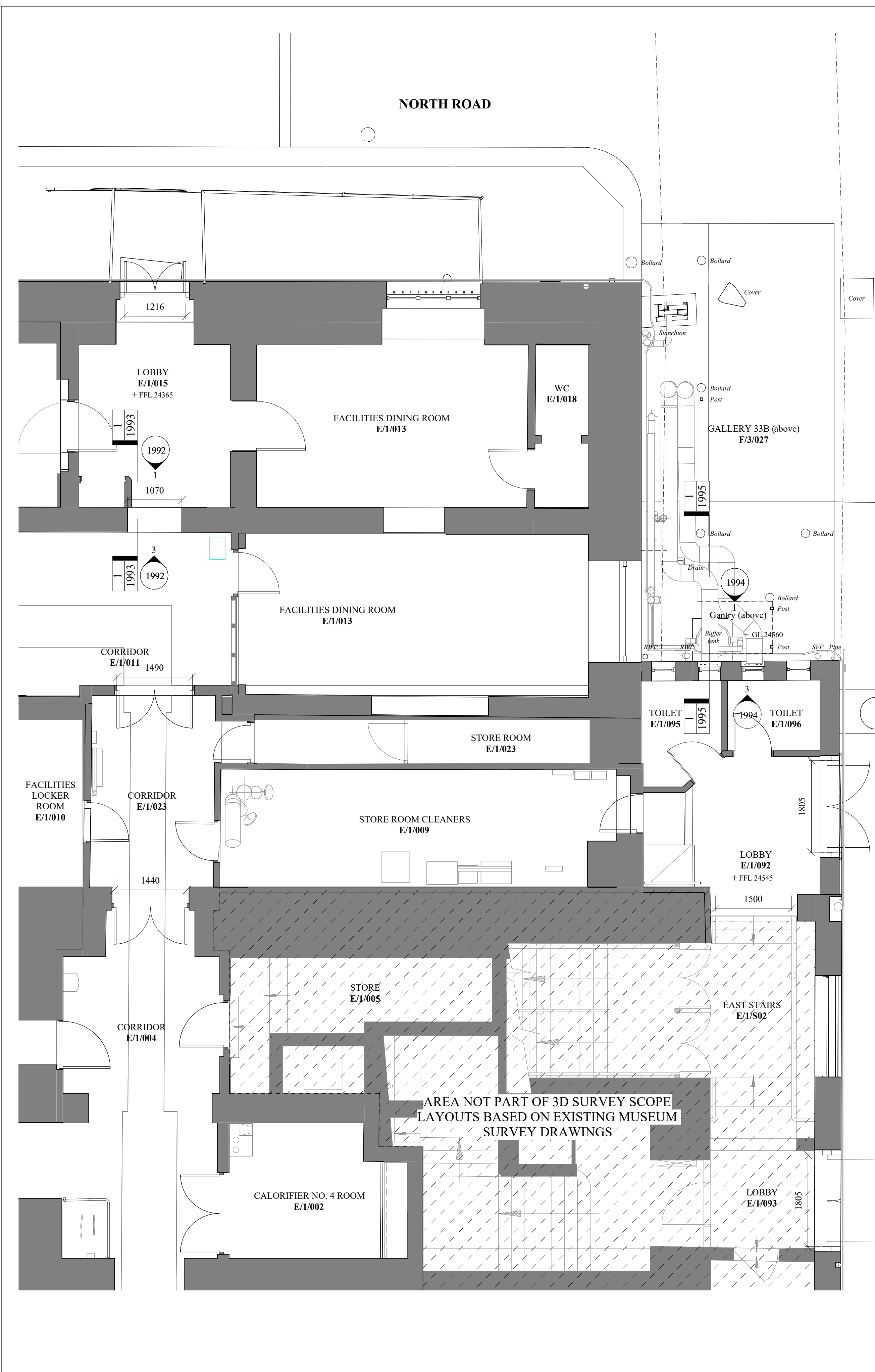
1 Level 1 North-East Plan - Existing
