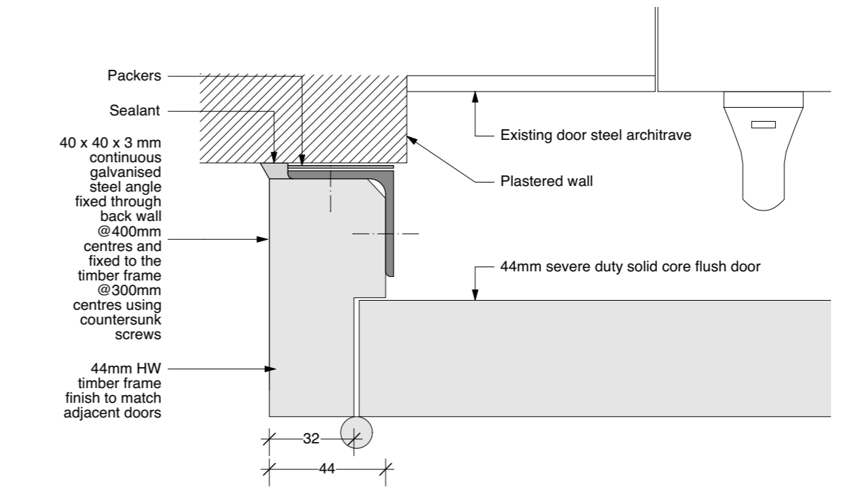
Plan detail Scale: Half Actual Size
