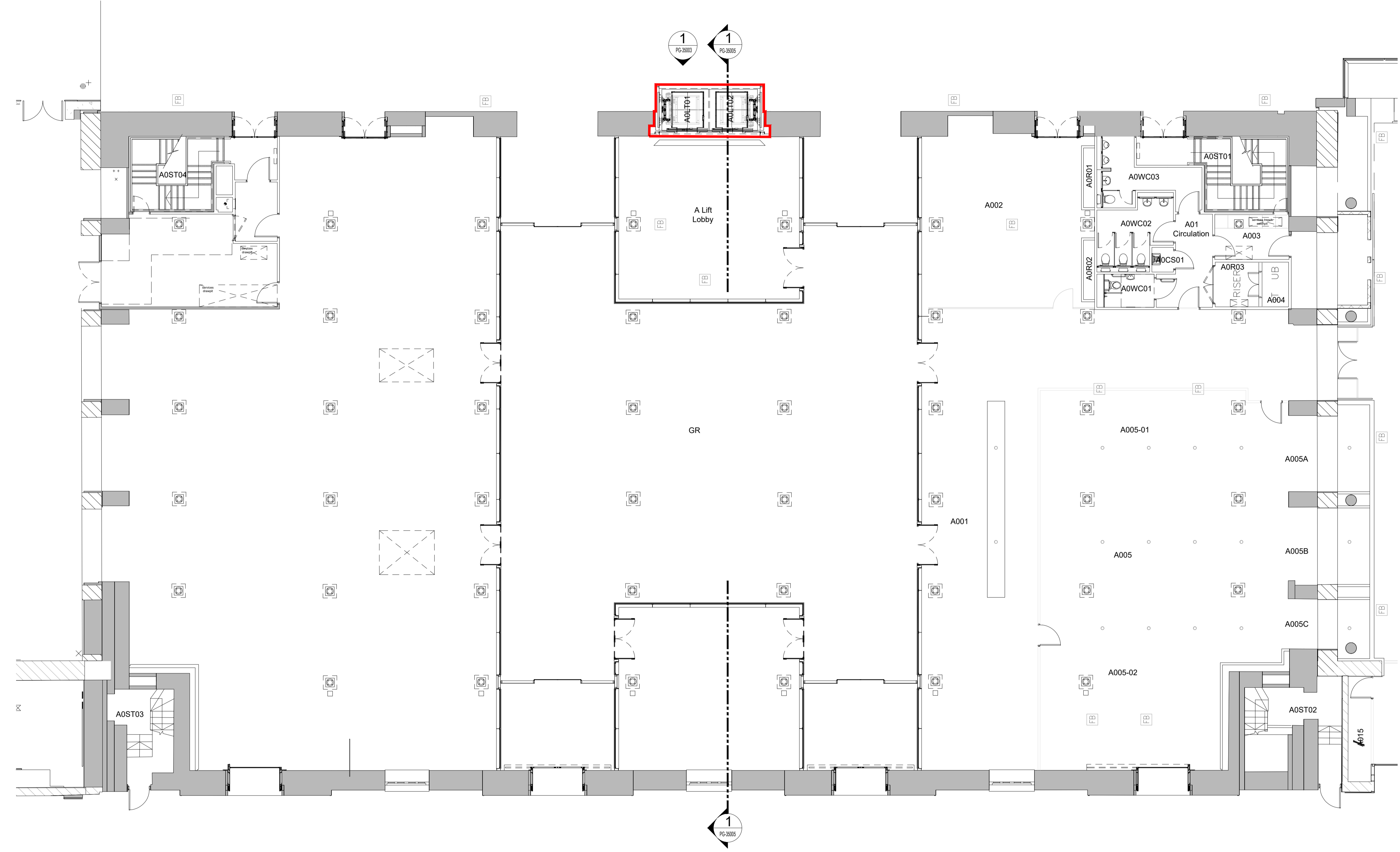
1 PROPOSED GROUND FLOOR GENERAL ARRANGEMENT 1:100
