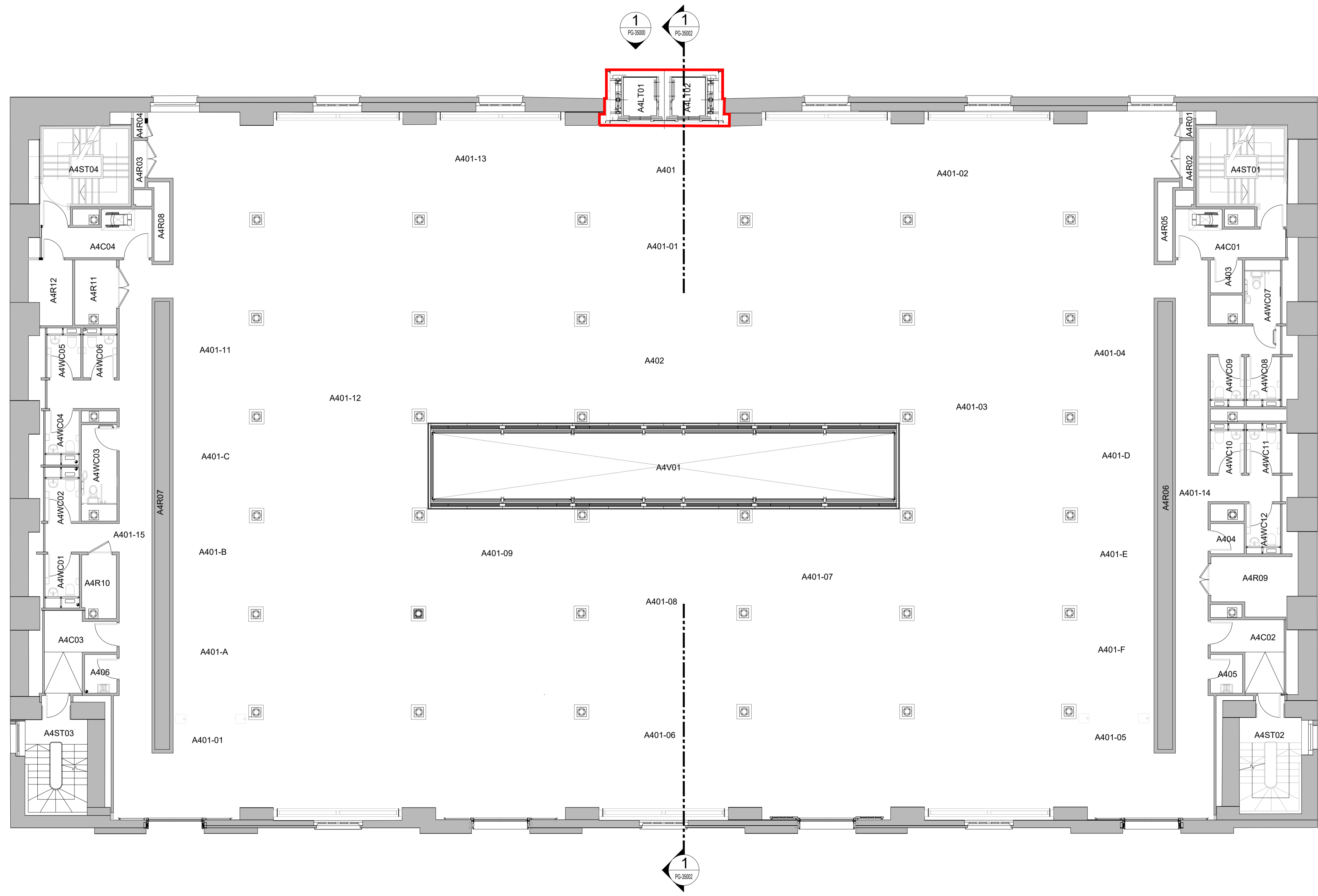
1 EXISTING 4TH FLOOR GENERAL ARRANGEMENT 1:100
