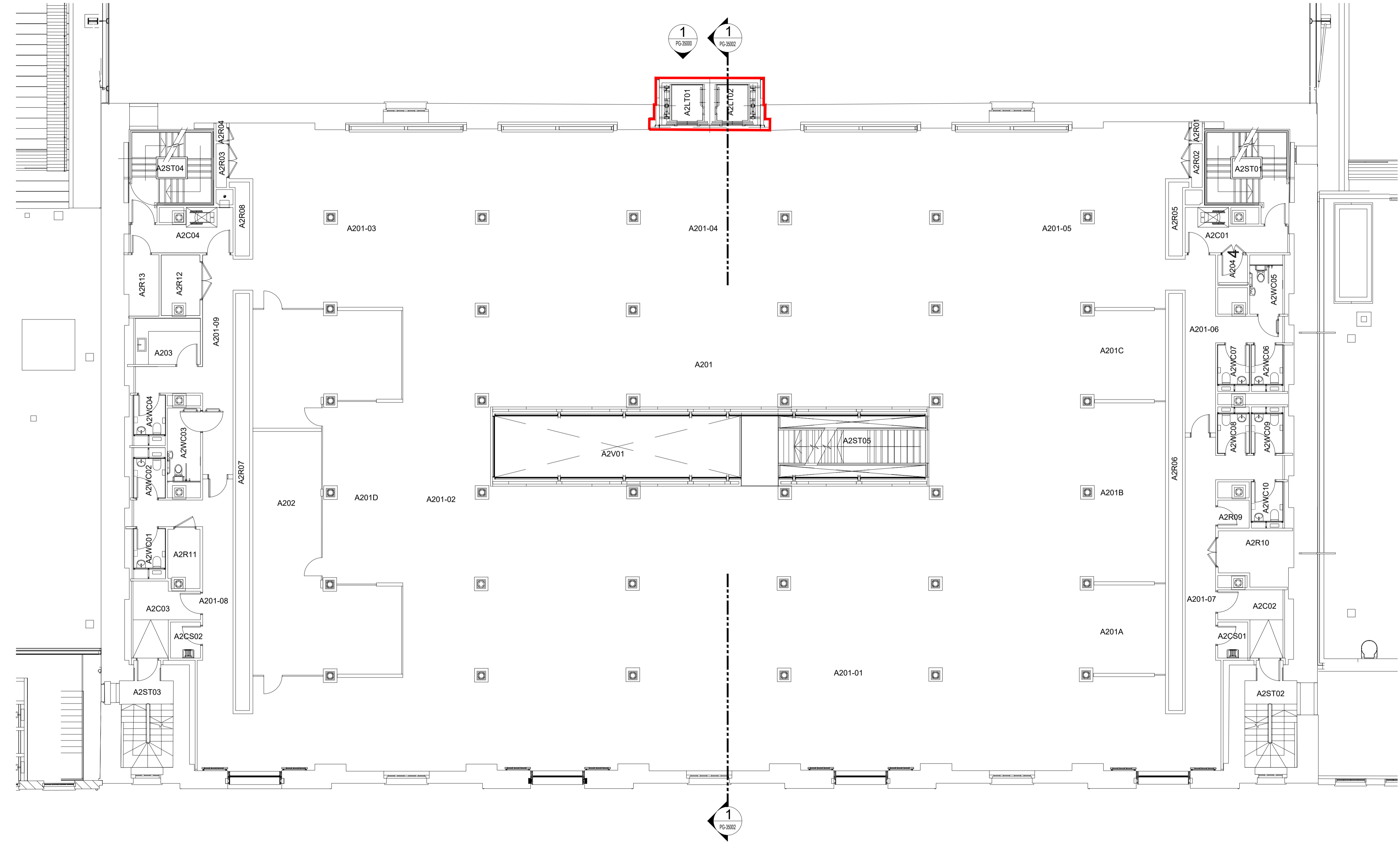
1 EXISTING 2ND FLOOR GENERAL ARRANGEMENT 1:100
