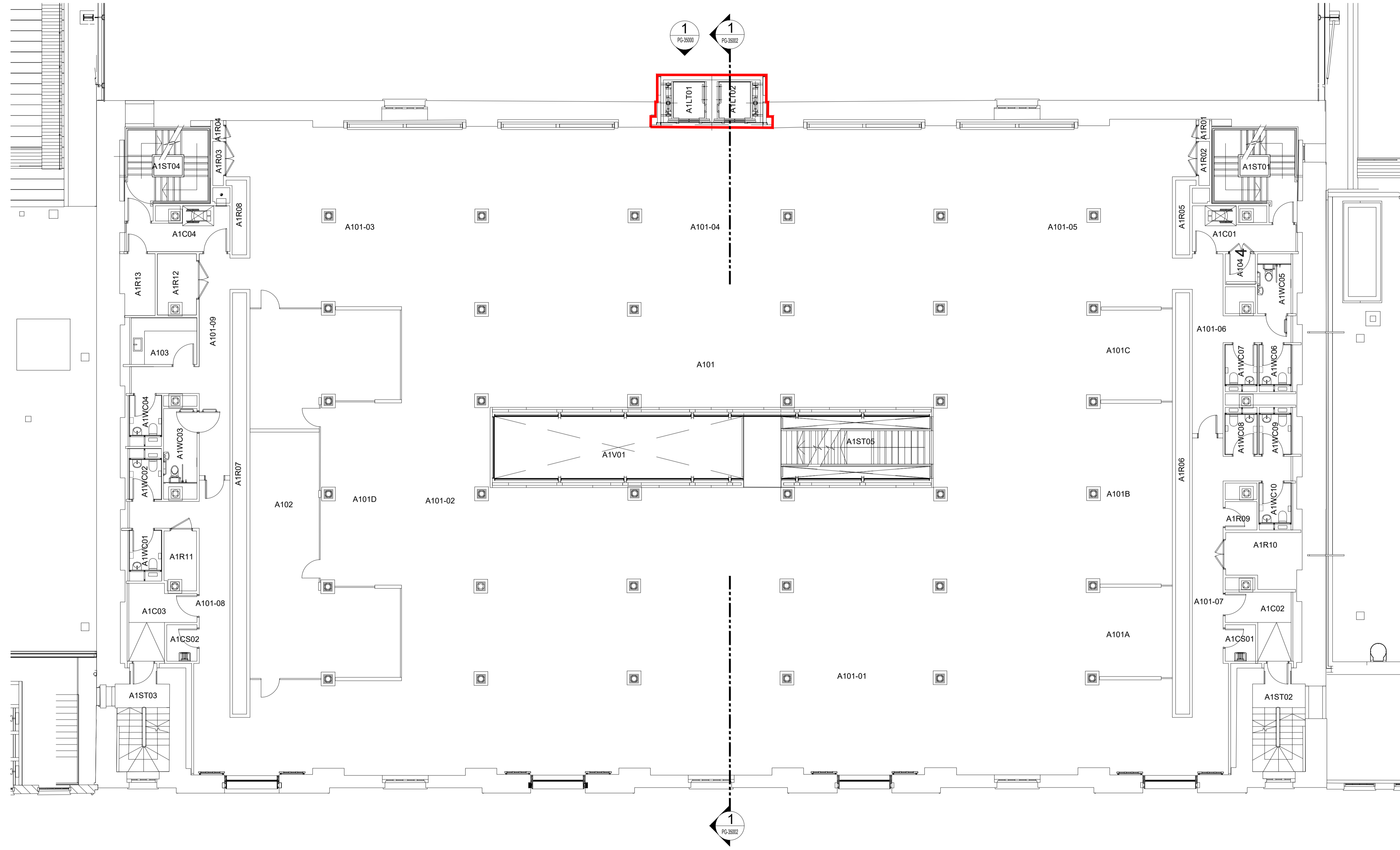
1 EXISTING 1ST FLOOR GENERAL ARRANGEMENT 1:100
