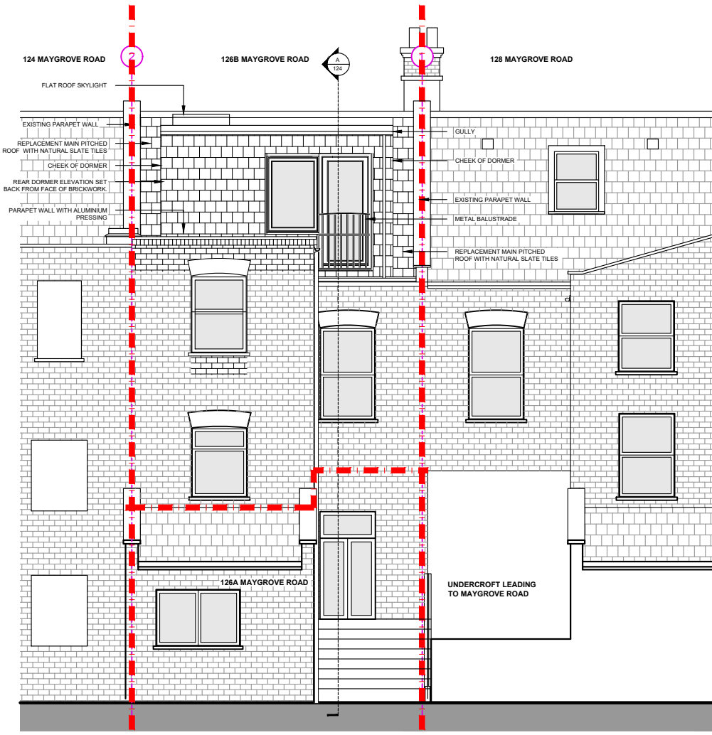
1 PROPOSED REAR ELEVATION 1: 100 @ A3
