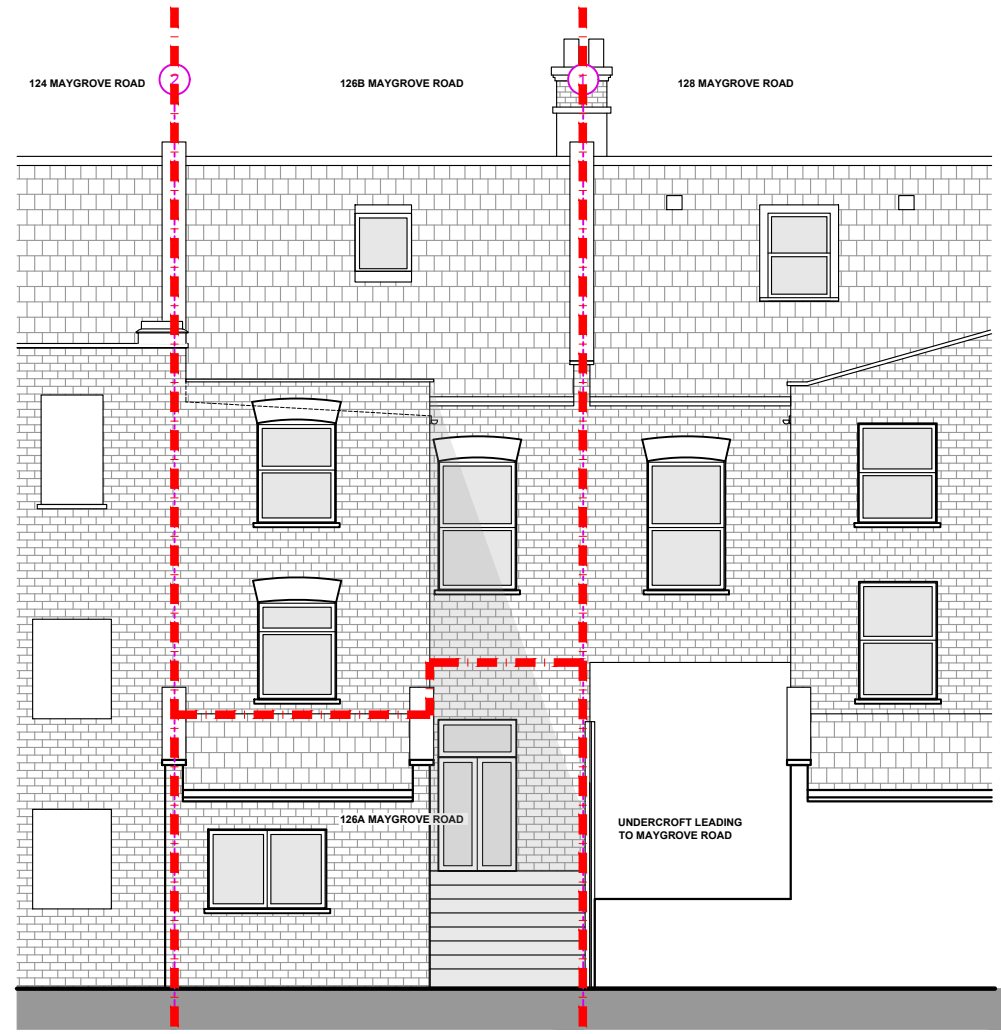
1 EXISTING REAR ELEVATION 1: 100 @ A3
