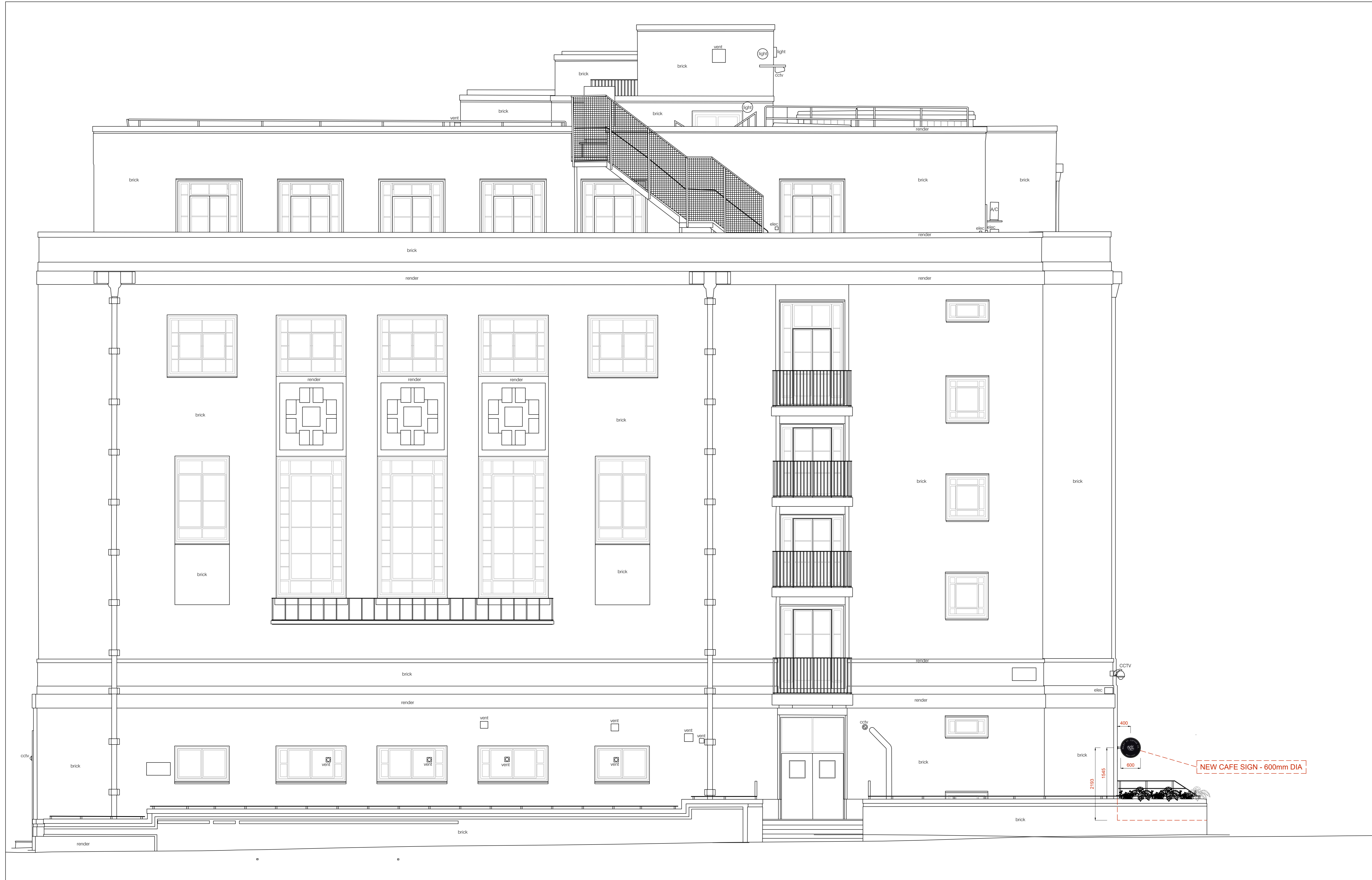
Proposed North Elevation
