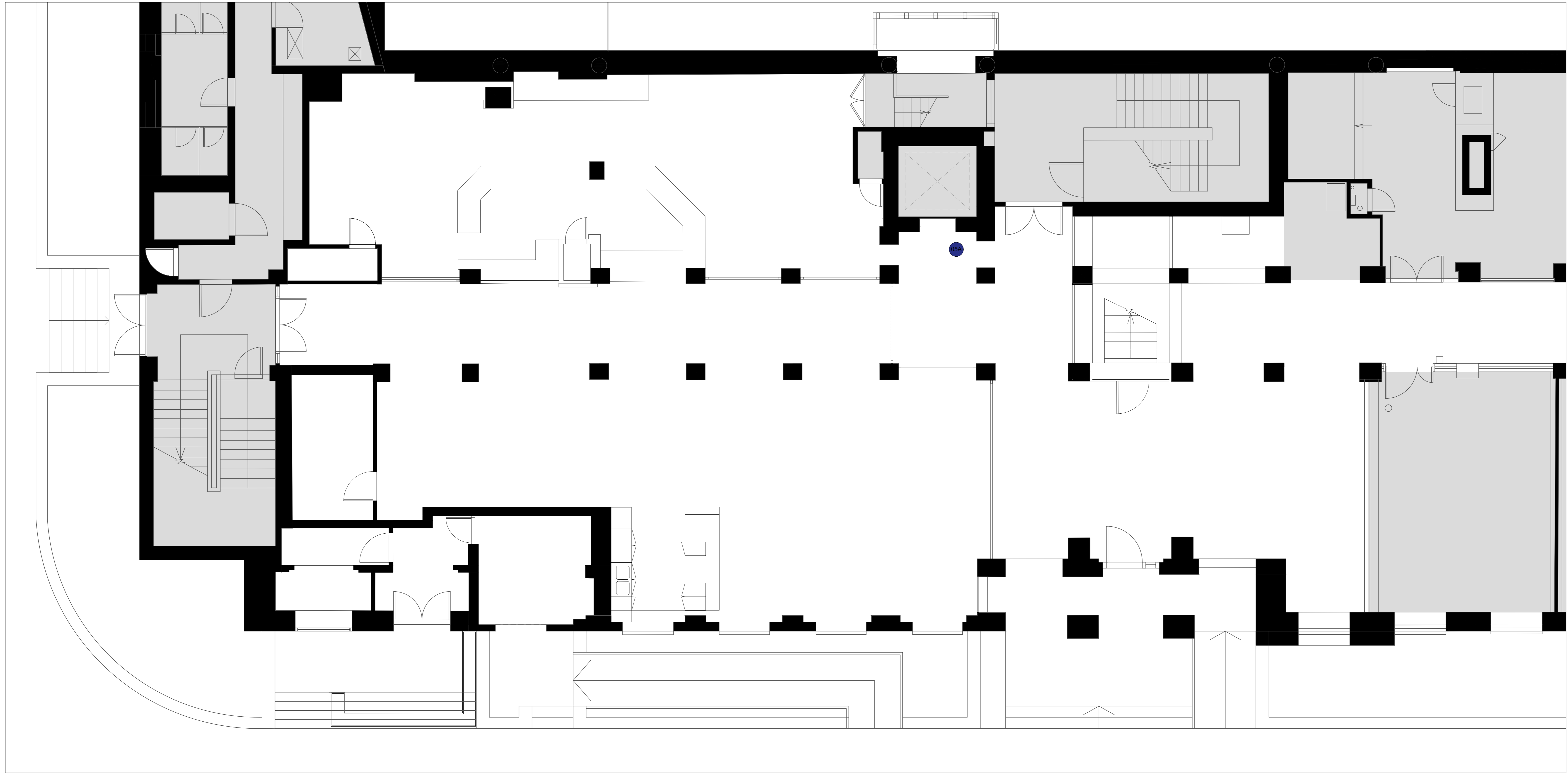
Existing Ground Floor GA - Scale 1:50
