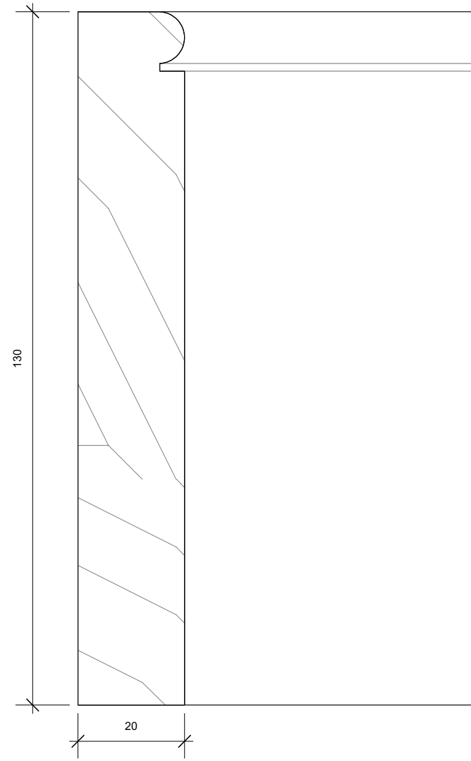
2 Skirting detail (43)01 Scale: Actual Size
