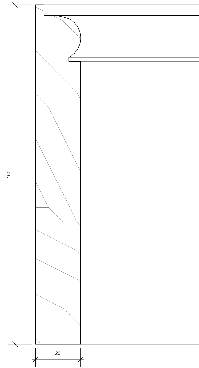
1 Skirting detail (43)01 Scale: Actual Size
