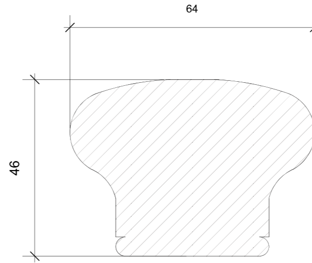
1 Handrail detail (24)02 Scale: 1:1@A3
