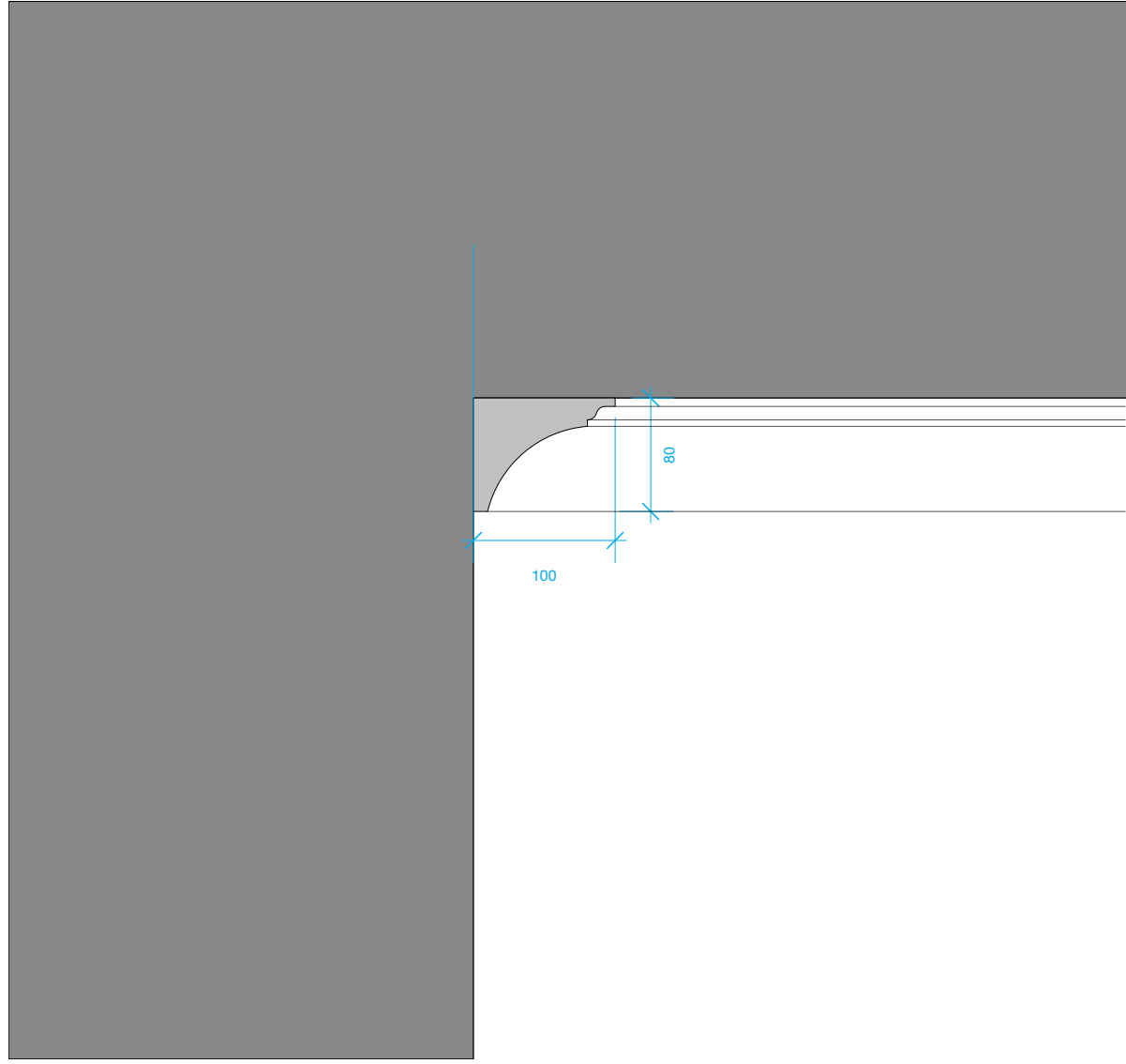
1 Second Floor Cornice 1:5
