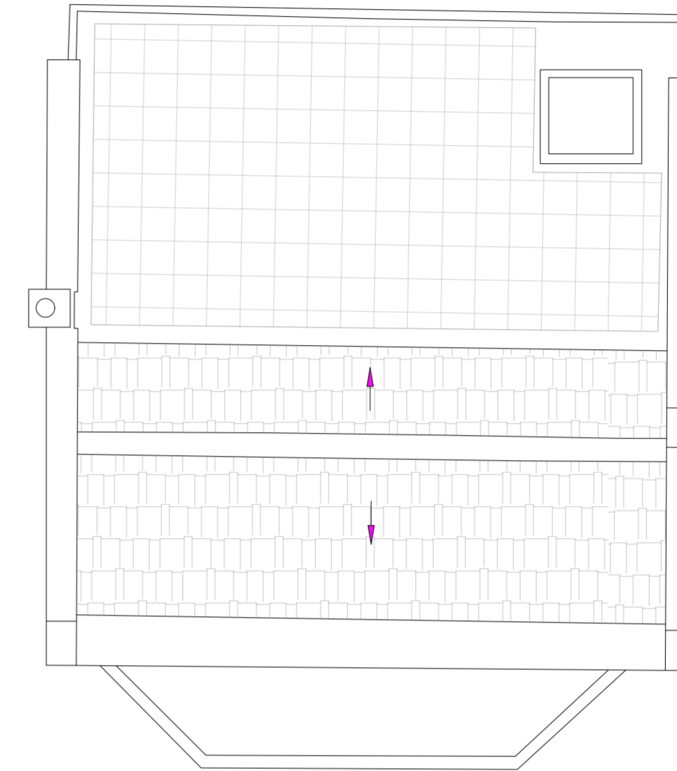
8 Proposed Roof Plan 102 Scale: 1:50
