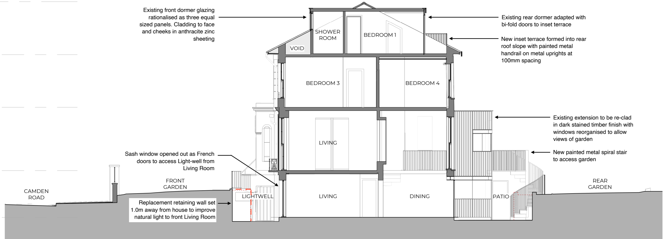
Proposed Section A
