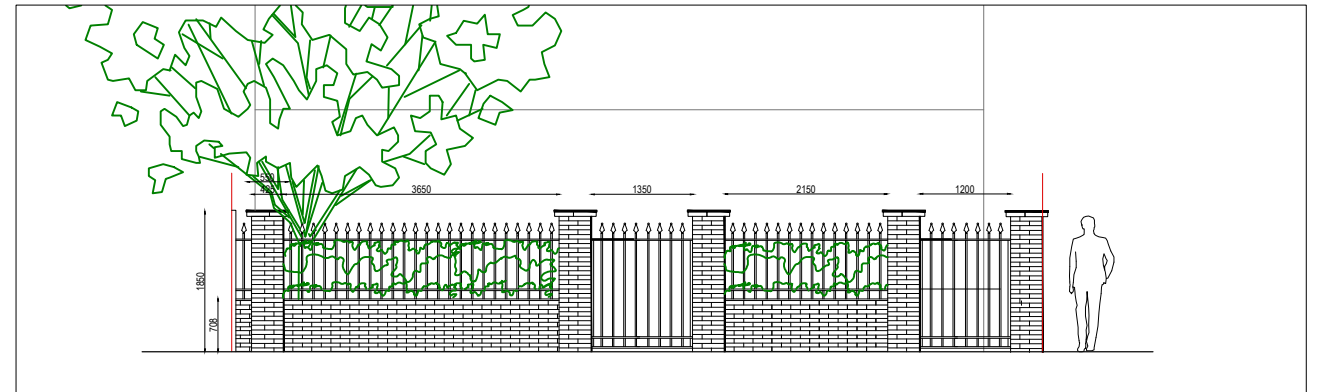
3 Proposed Gate Elevation scale 1:100
