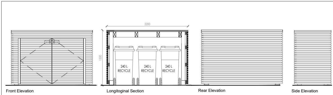
4 Proposed Refuse Storage scale 1:50
