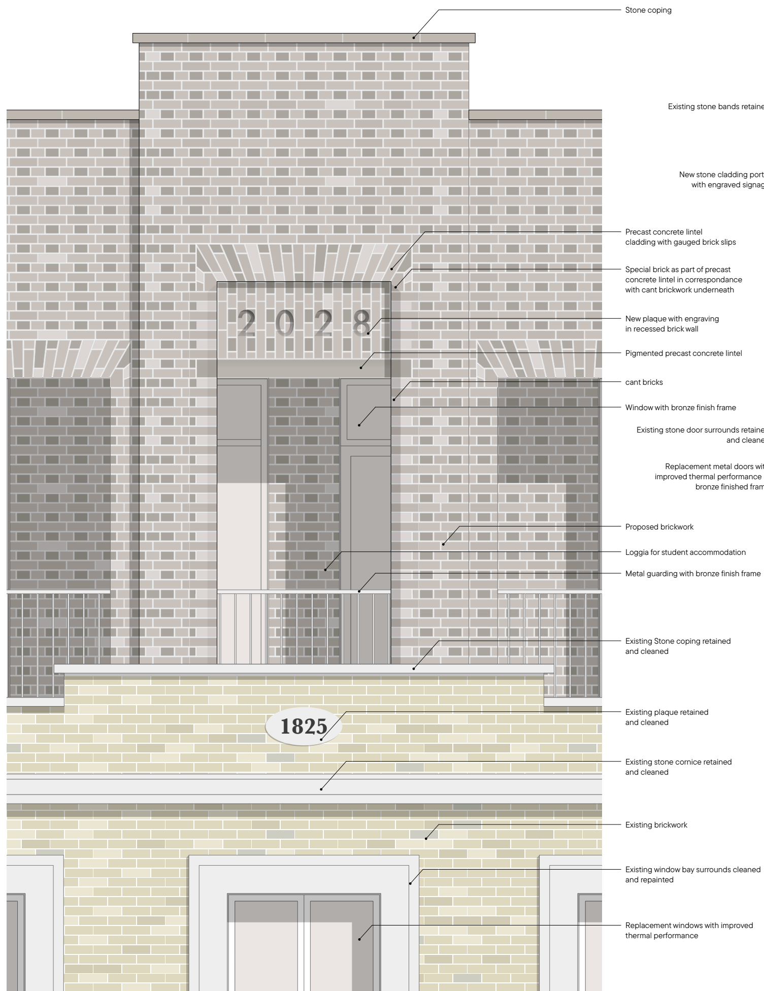
PROPOSED ELEVATION DETAIL 01
