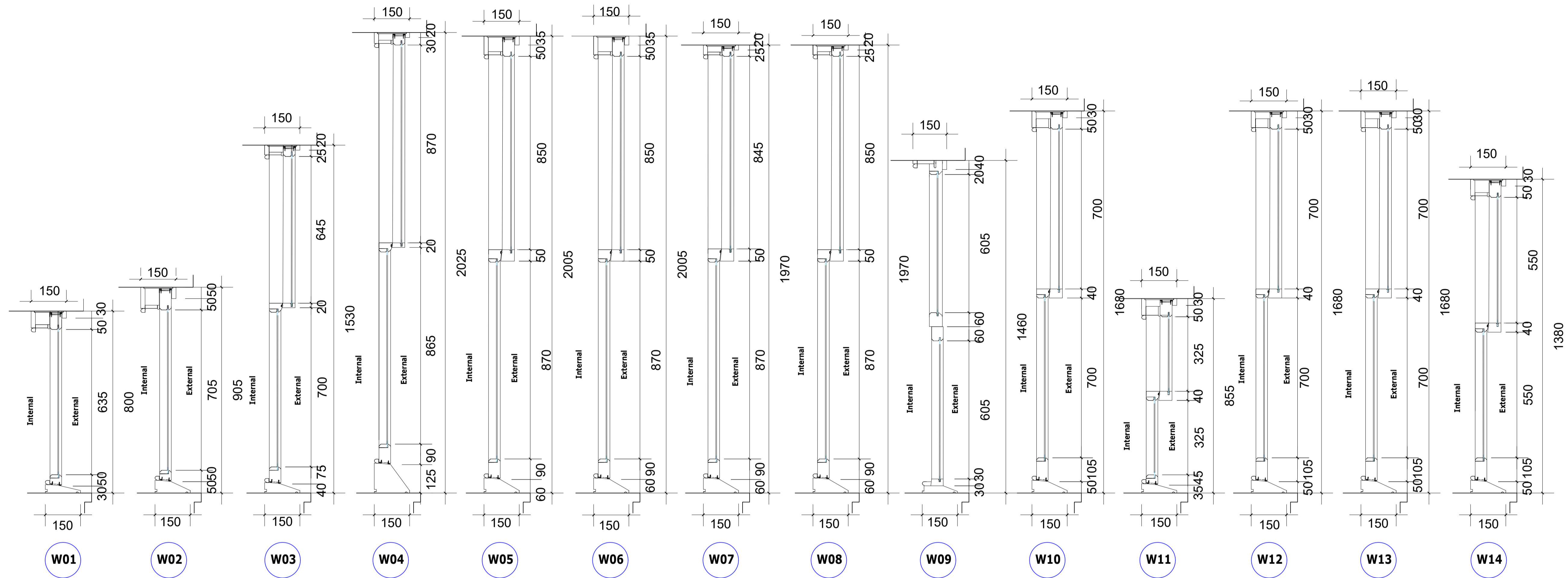
1 Existing Window Section Details Scale: 1:10 @ A1
