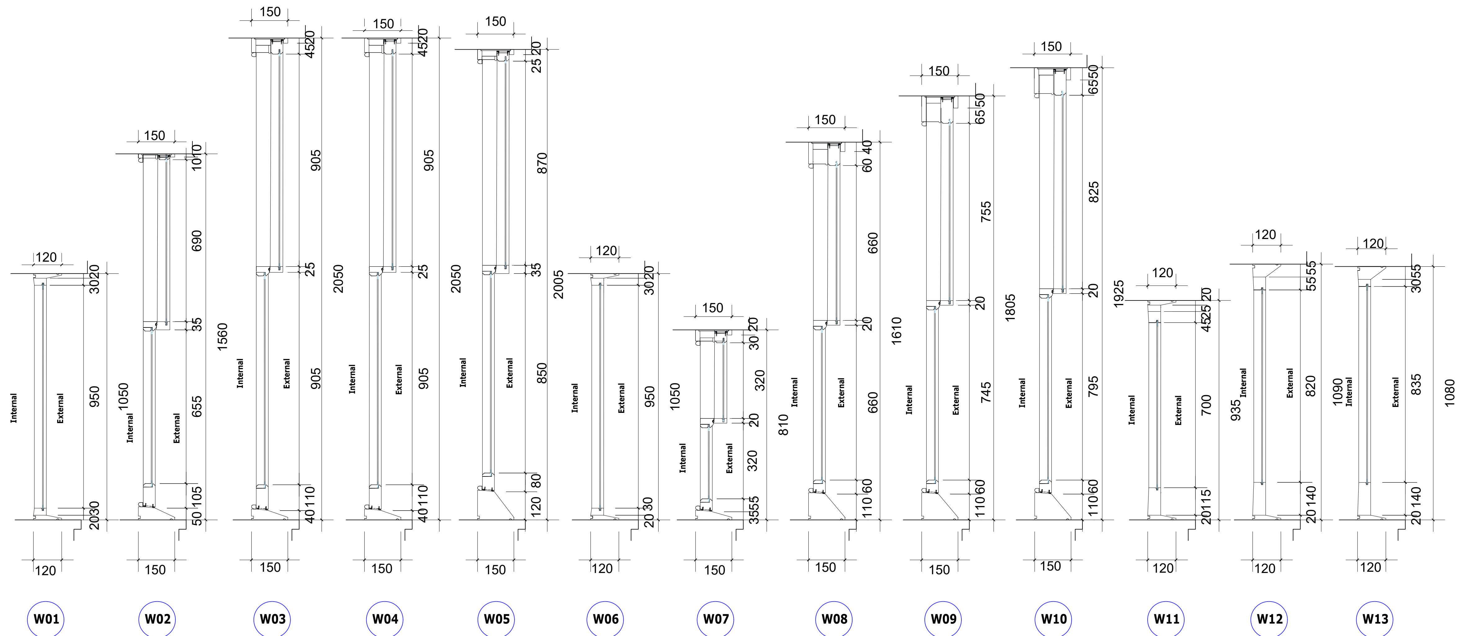
1 Existing Window Section Details Scale: 1:10 @ A1
