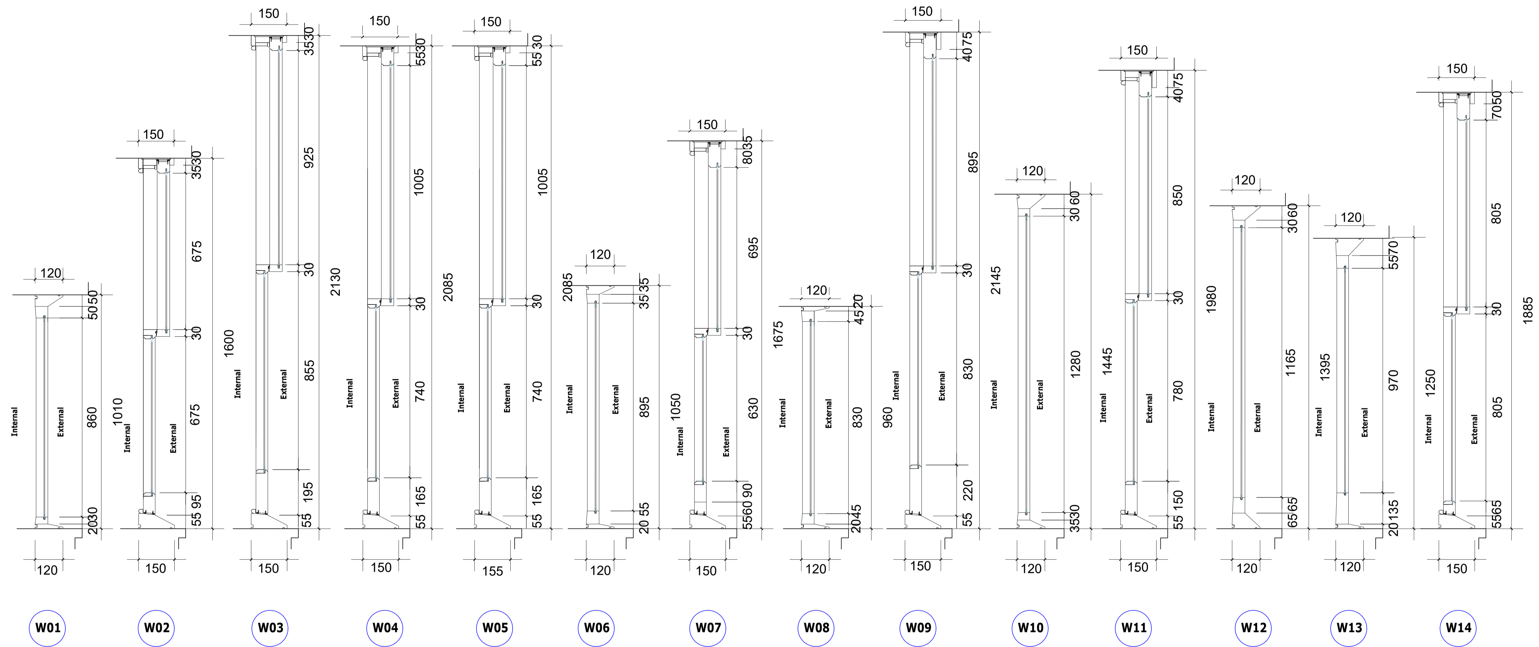
1 Existing Window Section Details Scale: 1:10 @ A1
