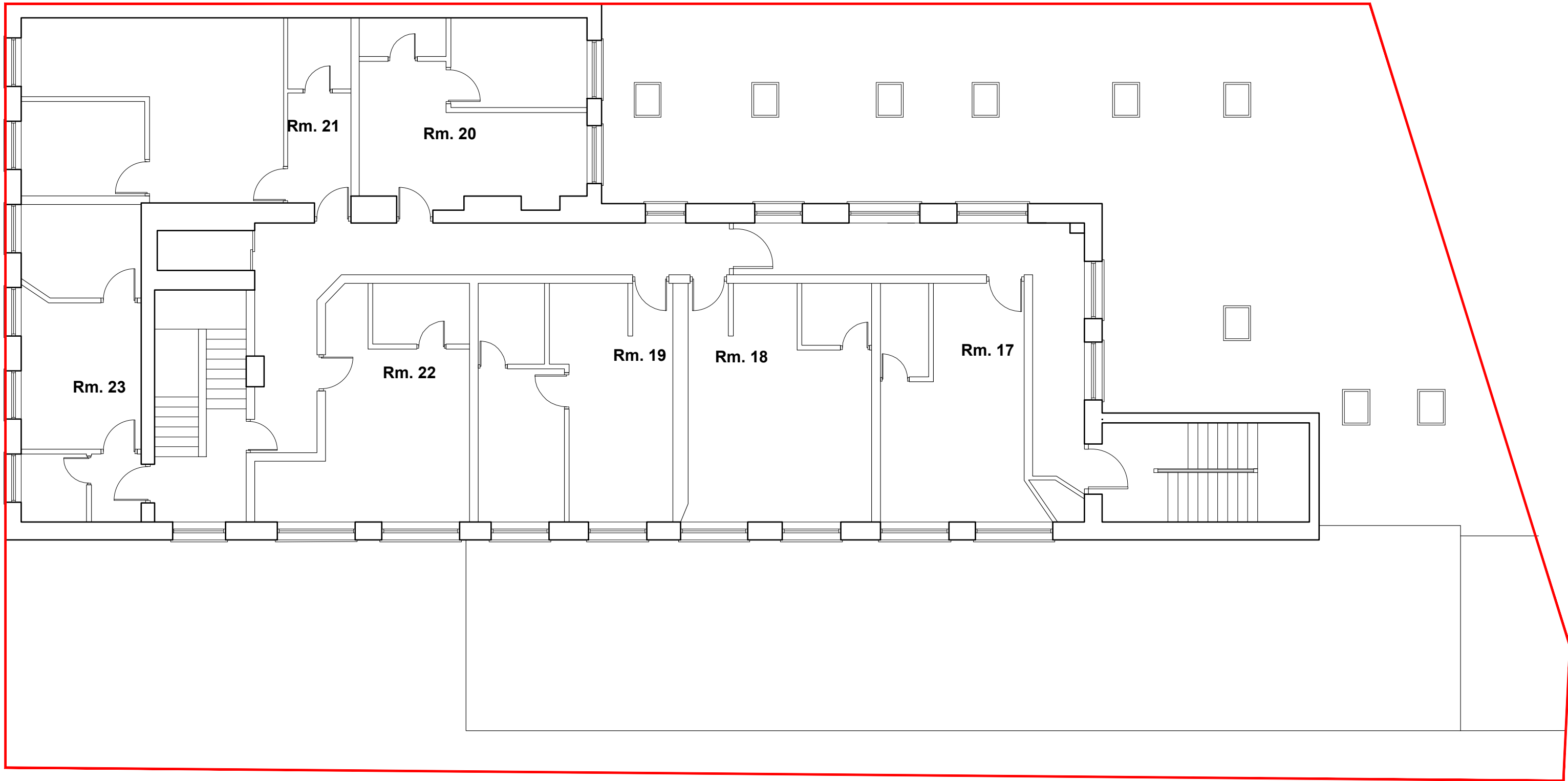
1. Existing First Floor Plan Scale: 1/100
