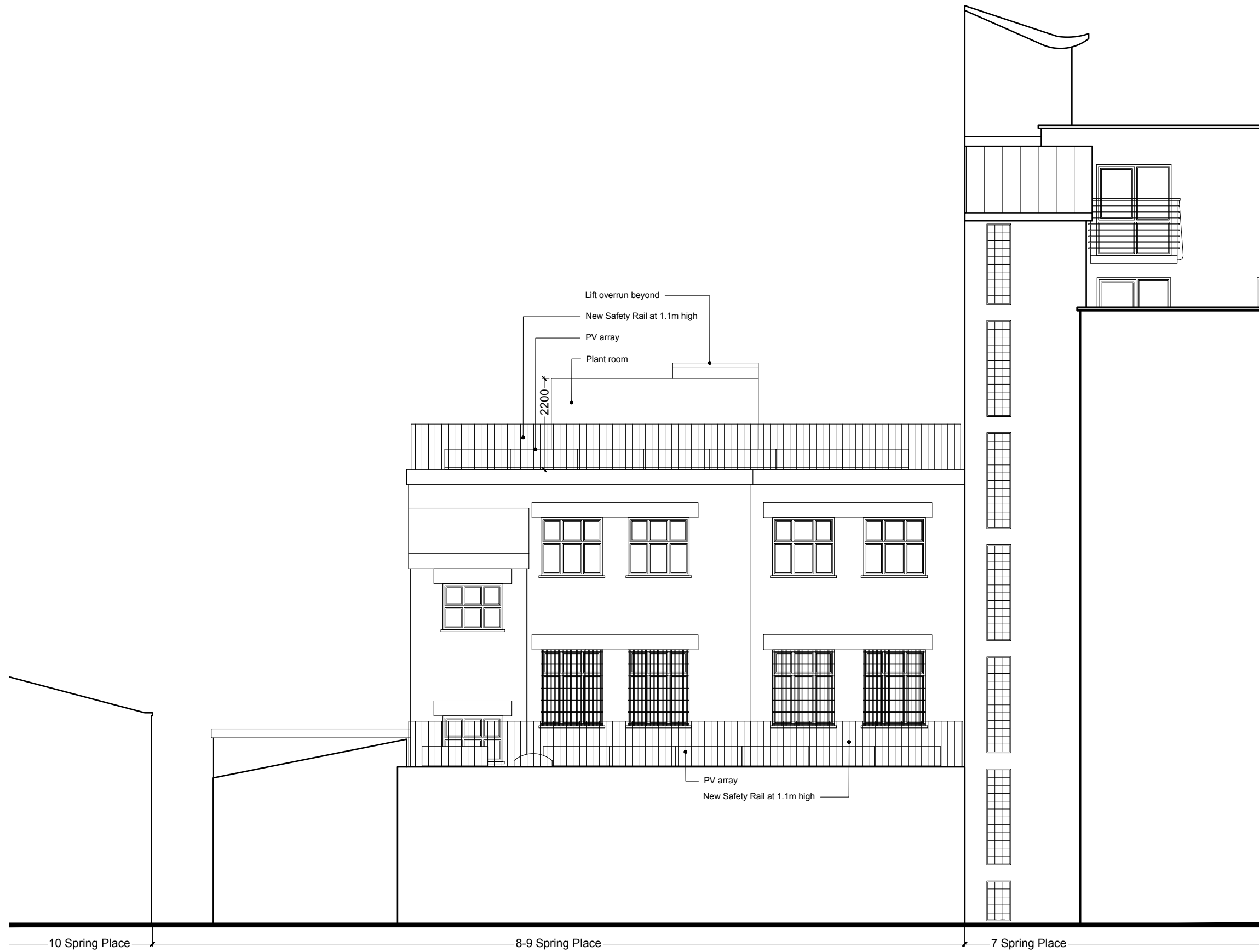
1. Proposed Rear Elevation Scale: 1/100
