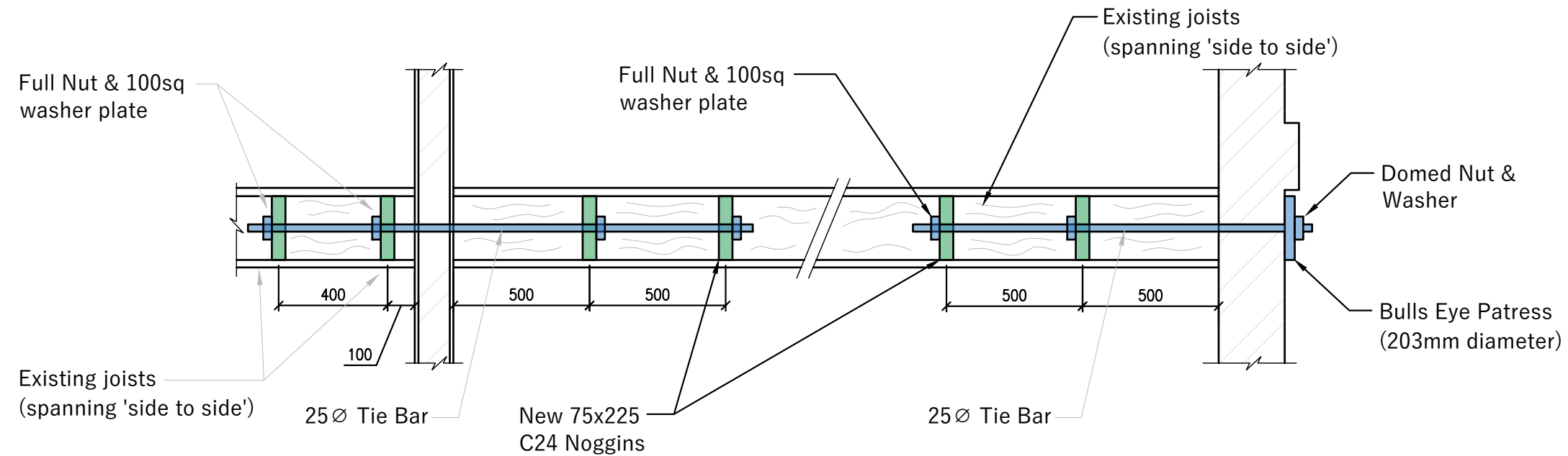
Section Through First Floor Sucwing Patress/Tie Bars (Scale 1:20)
