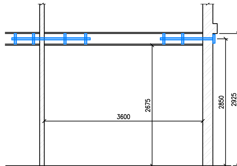
Typical Section Through Office & Lounge (Scale 1:50)
