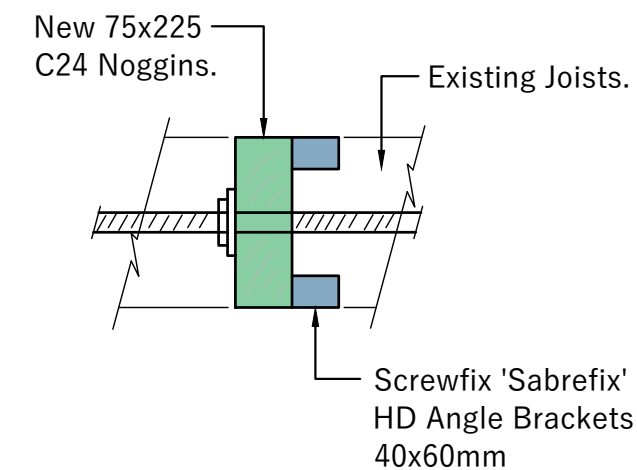
Connection Between New Noggins & Existing Joists (Scale 1:10)
