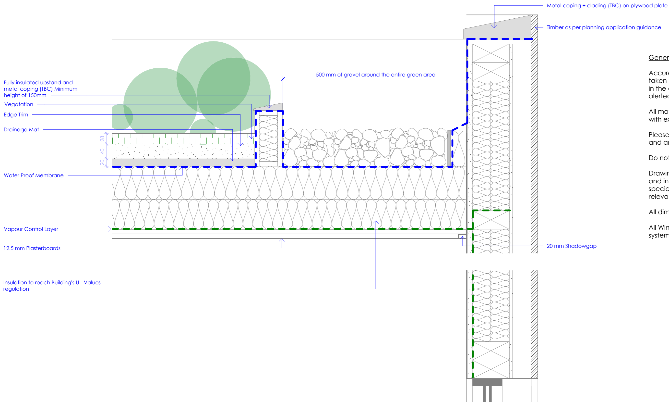
Extensive Green Roof Detail 1 : 5
